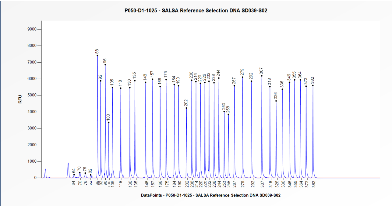
Figure 1. Capillary electrophoresis pattern from SALSA Reference Selection DNA SD039-S02 (approximately 50 ng) analysed with SALSA MLPA Probemix P050 CAH (D1-1025).
