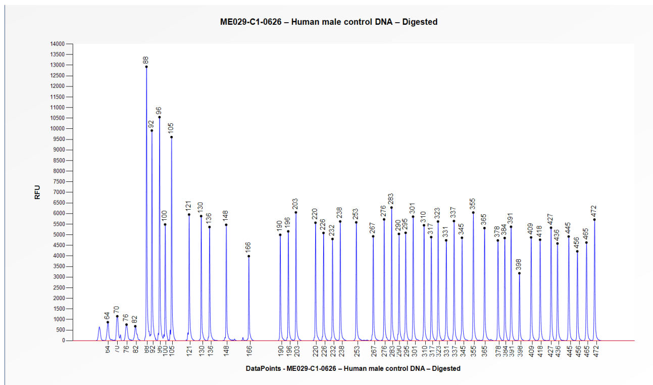
Figure 2. Capillary electrophoresis pattern from a sample of approximately 50 ng digested human male control DNA analysed with ME029 FMR1-AFF2 (C1-0626) to determine the methylation status.
