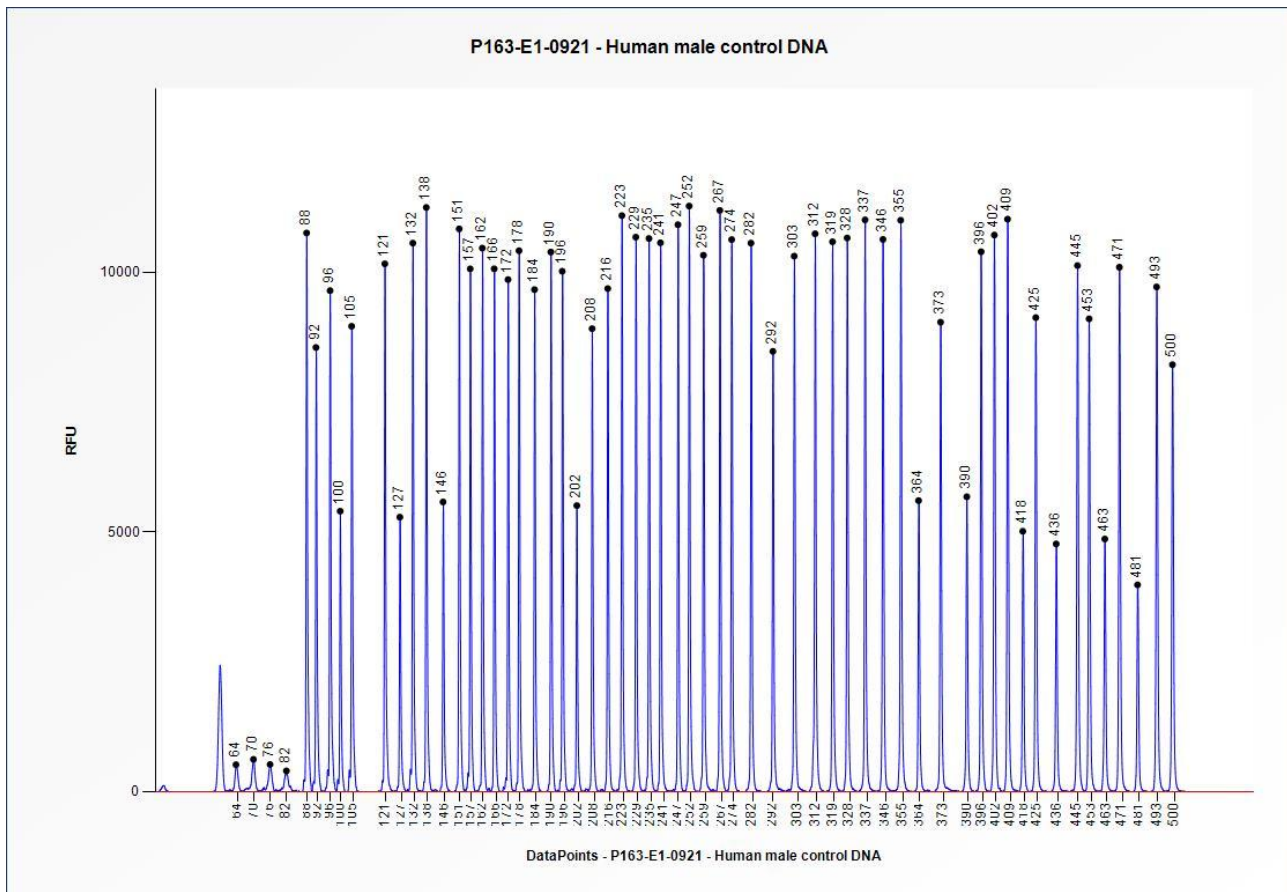
Figure 1. Capillary electrophoresis pattern from a sample of approximately 50 ng human male control DNA analysed with SALSA MLPA Probemix P163 GJB-WFS1-POU3F4 (E1-0921).
