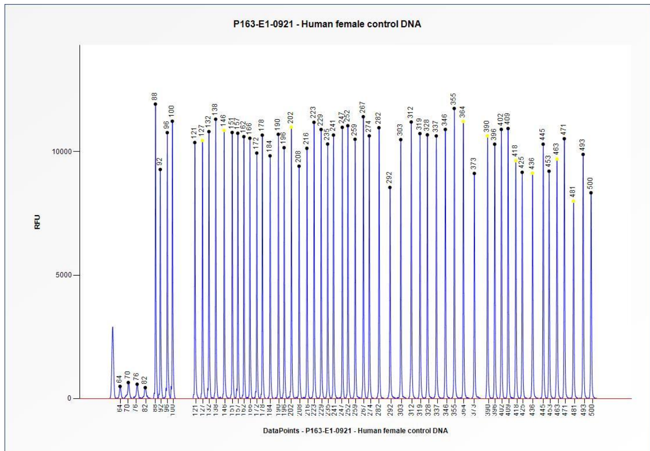
Figure 2 Capillary electrophoresis pattern from a sample of approximately 50 ng human female control DNA analysed with SALSA MLPA Probemix P163 GJB-WFS1-POU3F4 (E1-0921).
