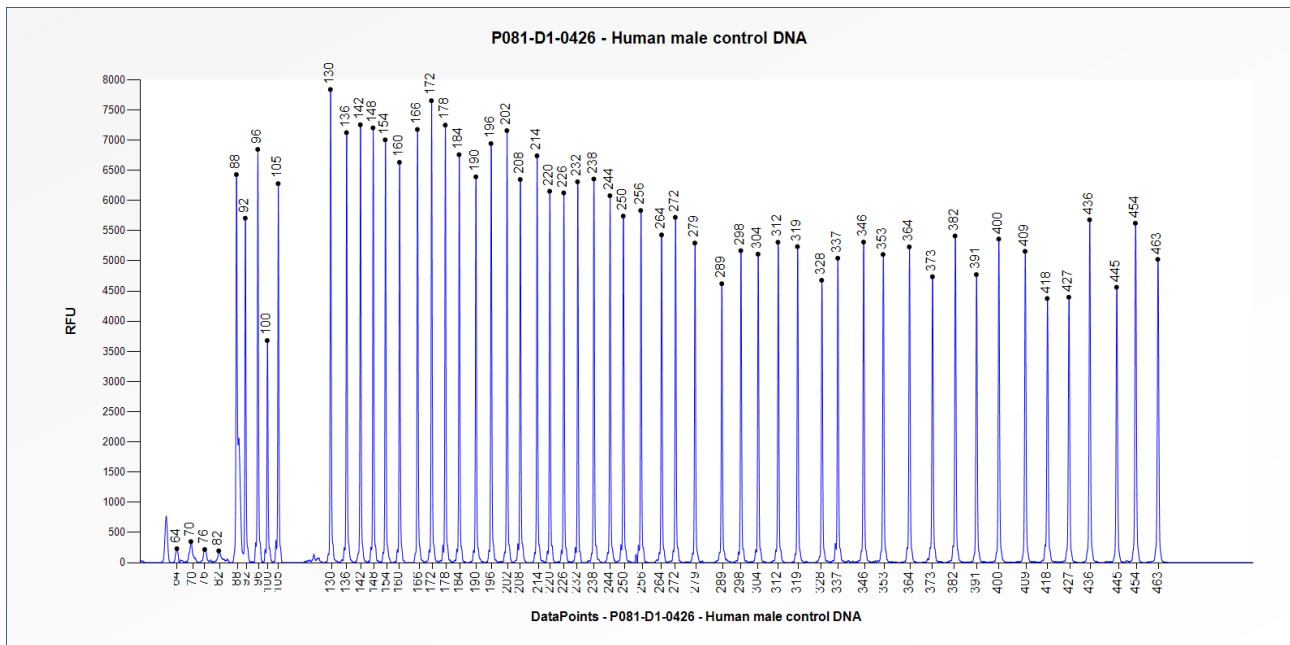
Figure 1. Capillary electrophoresis pattern from a sample of approximately 50 ng human male control DNA analysed with P081 NF1 mix 1 (D1-0426).
