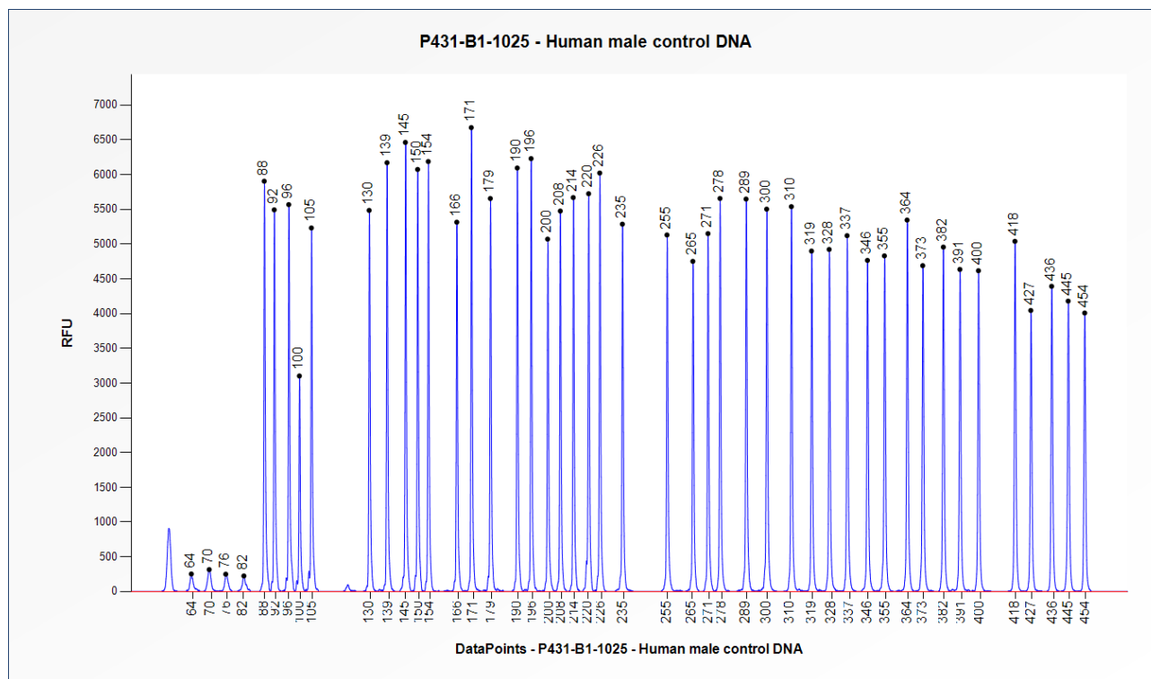
Figure 1. Capillary electrophoresis pattern from a sample of approximately 50 ng human male control DNA analysed with P431 FOXF1 (B1-1025).
