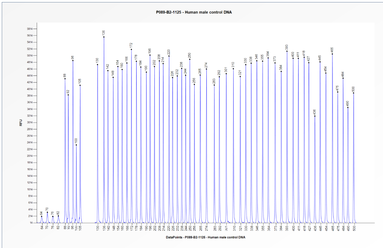
Figure 1. Capillary electrophoresis pattern from a sample of approximately 50 ng human male control DNA analysed with P089 TK2 (B2-1125).
