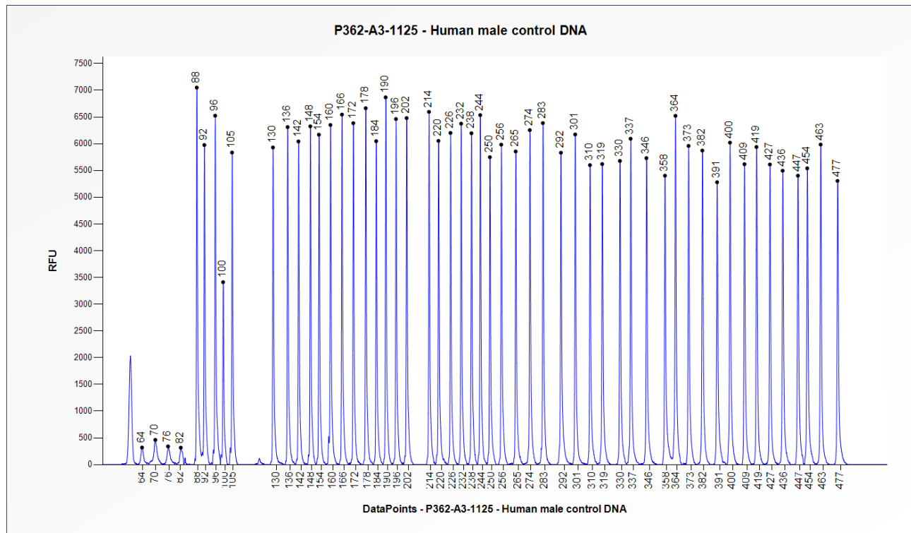
Figure 1. Capillary electrophoresis pattern from a sample of approximately 50 ng human male control DNA analysed with P362 USH2A mix 2 (A3-1125).
