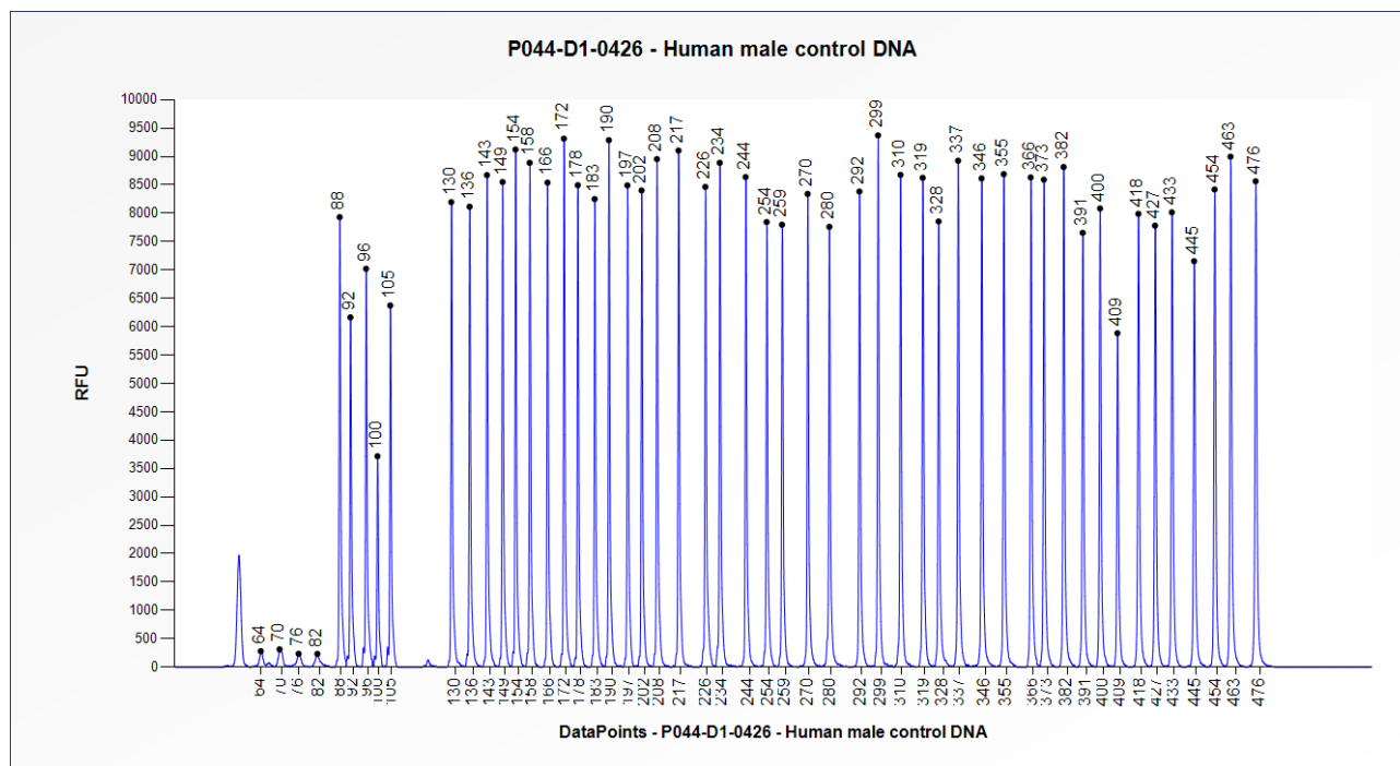
Figure 1. Capillary electrophoresis pattern from a sample of approximately 50 ng human male control DNA analysed with P044 NF2 (D1-0426).
