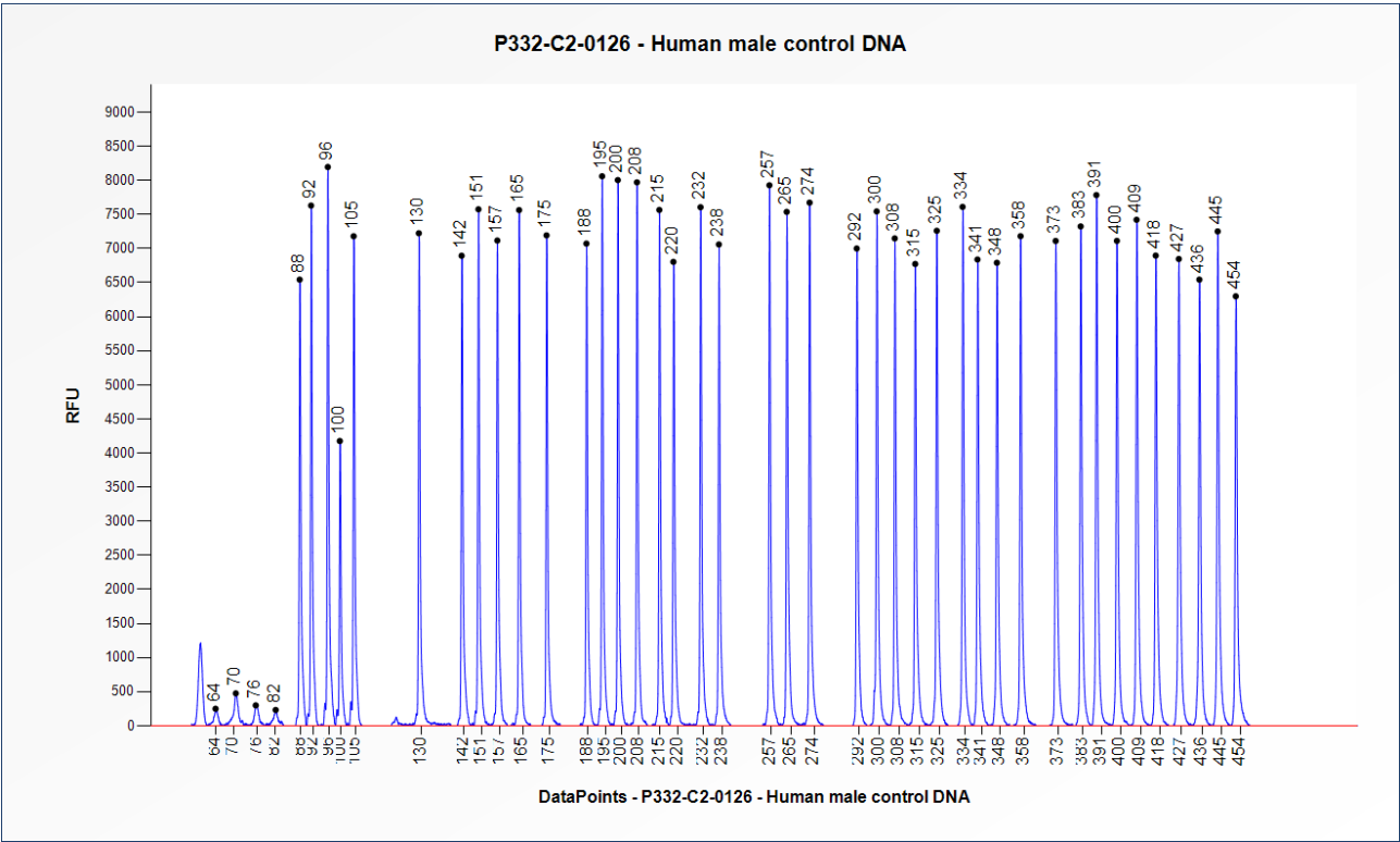
Figure 1. Capillary electrophoresis pattern from a sample of approximately 50 ng human male control DNA analysed with P332 COL5A1 mix-2 (C2-0126).
