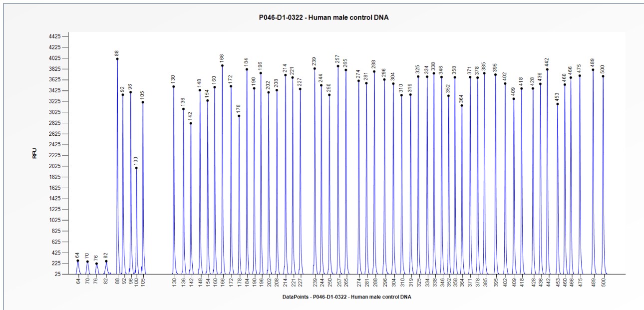
Figure 1. Capillary electrophoresis pattern from a sample of approximately 50 ng human male control DNA analysed with SALSA MLPA Probemix P046 TSC2 (D1-0322).
