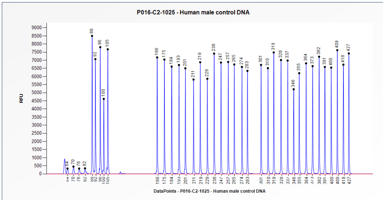
Figure 1. Capillary electrophoresis pattern from a sample of approximately 50 ng human male control DNA analysed with SALSA MLPA Probemix P016 VHL (C2-1025).
