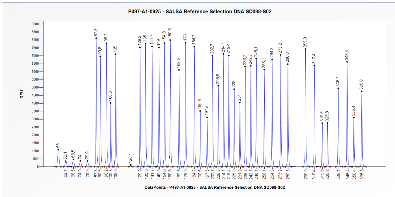
Figure 1. Capillary electrophoresis pattern from SALSA Reference Selection DNA SD098-S02 (approximately 50 ng) analysed with SALSA MLPA Probemix P497 Opsin (A1-0925).
