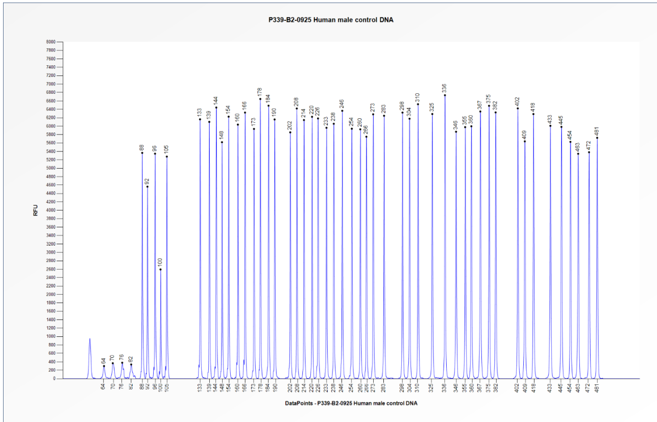
Figure 1. Capillary electrophoresis pattern from a sample of approximately 50 ng human male control DNA analysed with SALSA MLPA Probemix P339 SHANK3 (B2-0925).
