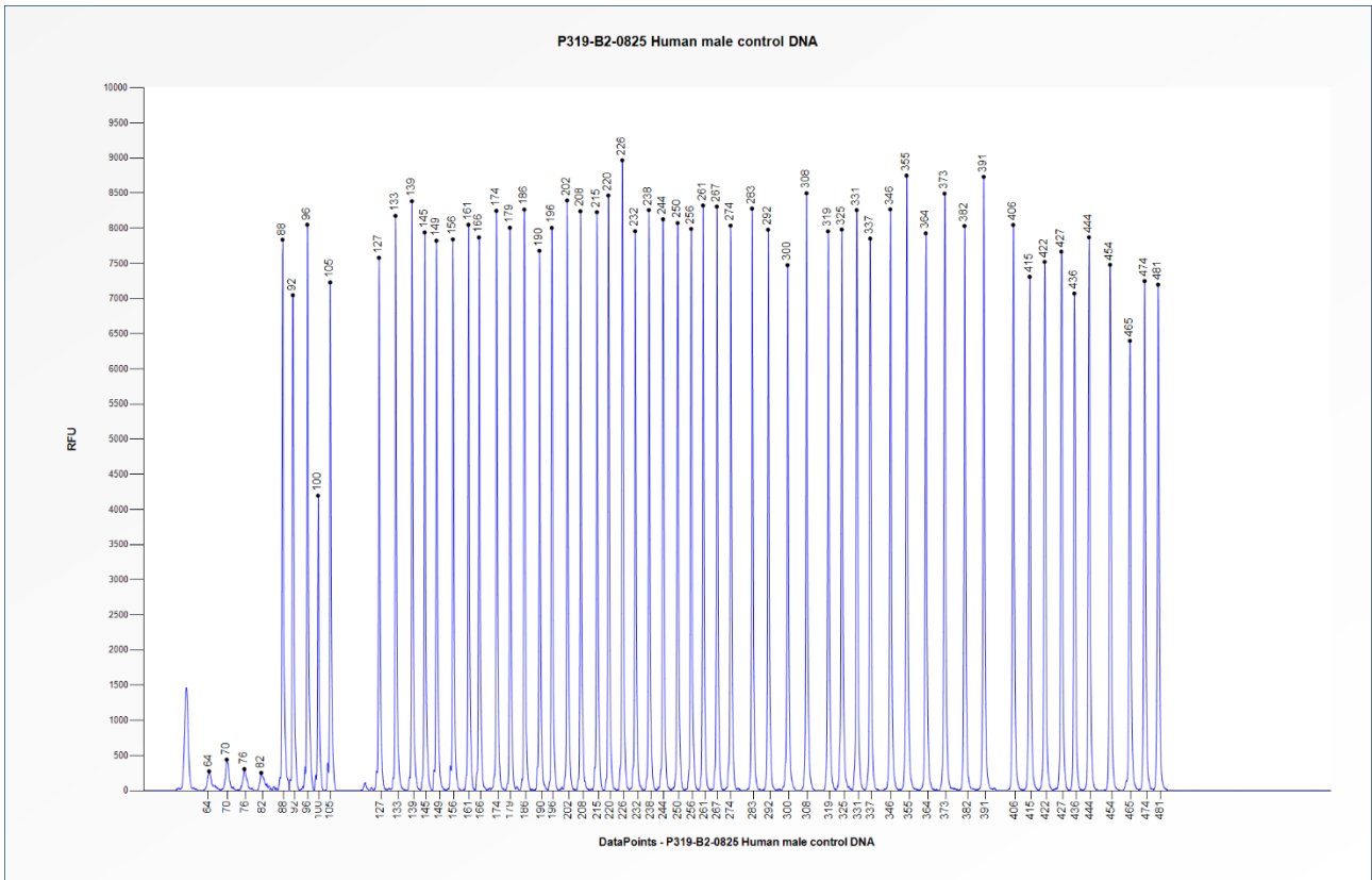
Figure 1. Capillary electrophoresis pattern from a sample of approximately 50 ng human male control DNA analysed with SALSA MLPA Probemix P319 Thyroid (B2-0825).
