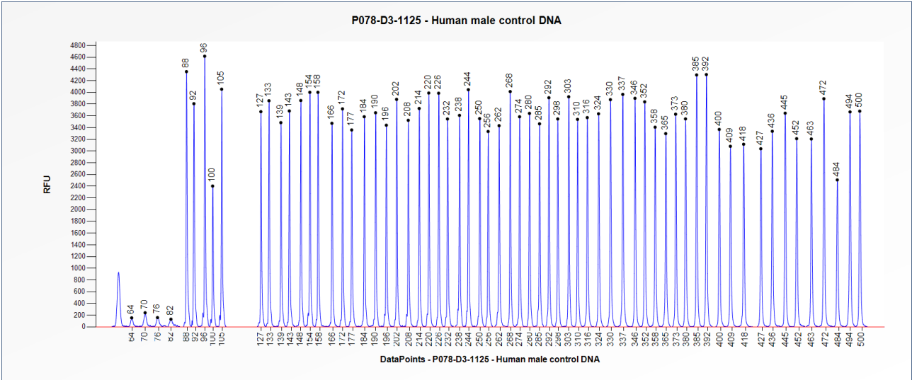
Figure 1. Capillary electrophoresis pattern from a sample of approximately 50 ng human male control DNA analysed with SALSA MLPA Probemix P078 Breast tumour (D3-1125).
