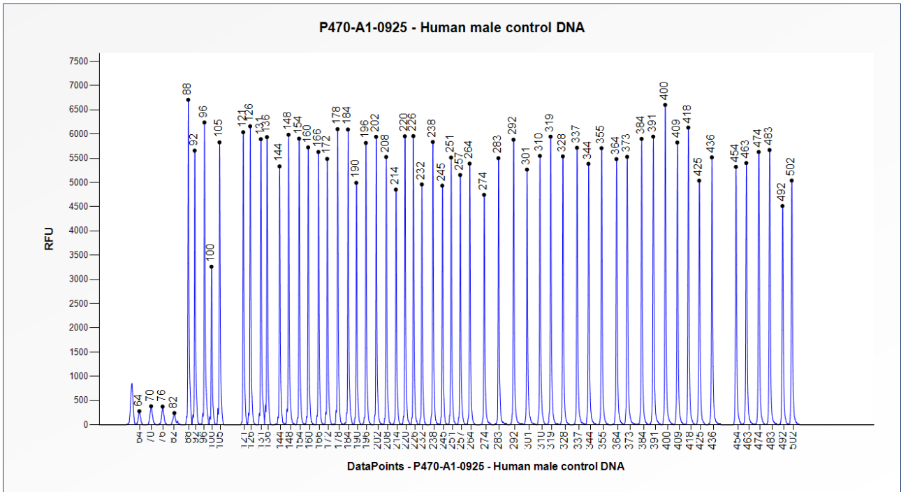
Figure 1. Capillary electrophoresis pattern from a sample of approximately 50 ng human male control DNA analysed with SALSA MLPA Probemix P470 NCL (A1-0925).
