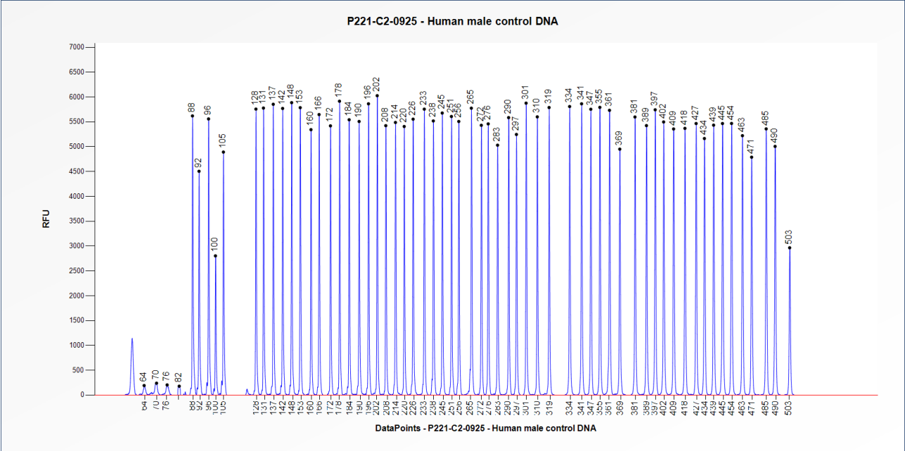
Figure 1. Capillary electrophoresis pattern from a sample of approximately 50 ng human male control DNA analysed with SALSA MLPA Probemix P221 LCA mix-1 (C2-0925).
