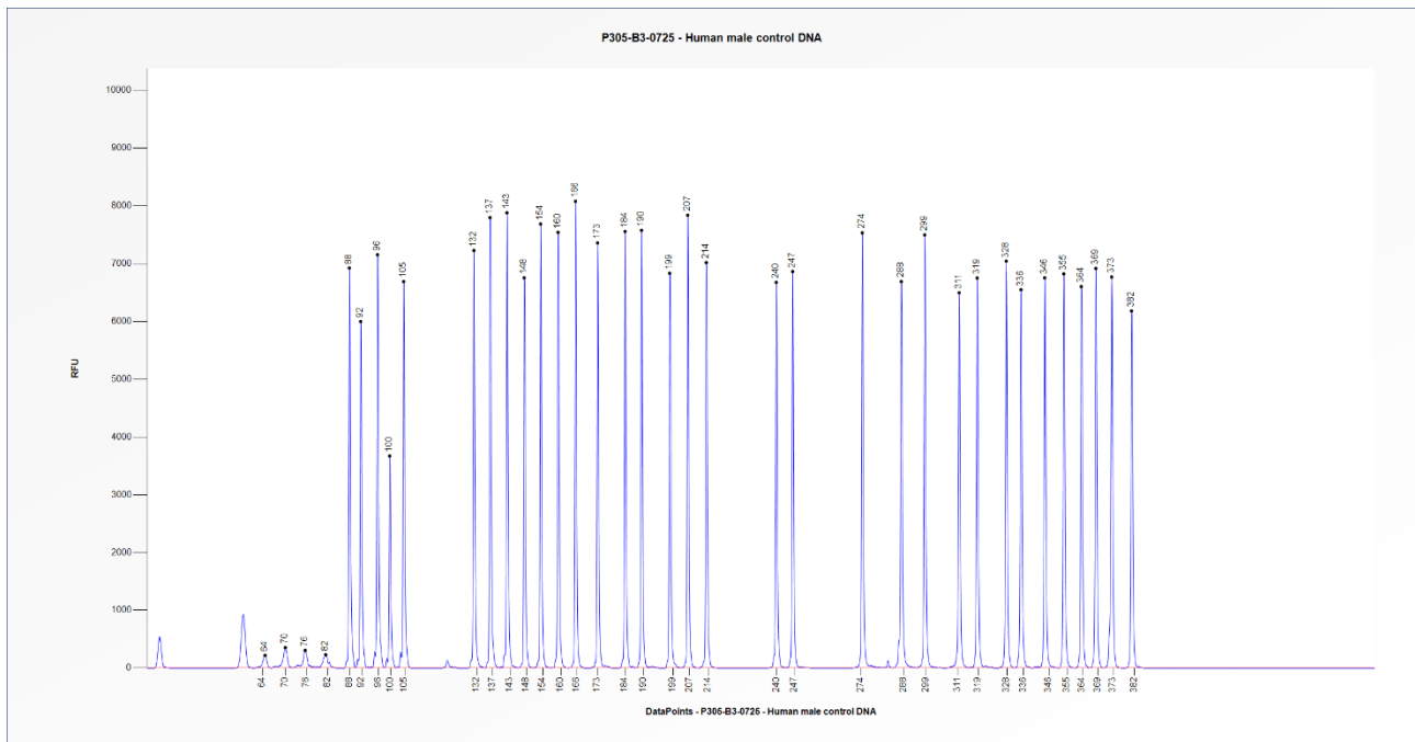
Figure 1. Capillary electrophoresis pattern from a sample of approximately 50 ng human male control DNA analysed with SALSA MLPA Probemix P305 AGXT (B3-0725).
