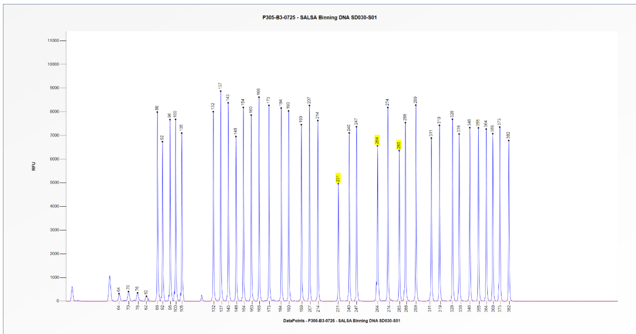
Figure 2. Capillary electrophoresis pattern from SALSA Binning DNA SD030-S01 (approximately 50 ng) analysed with SALSA MLPA Probemix P305 AGXT (B3-0725). The locations of the AGXT c.731T>C, c.33_34insC and c.508G>A specific probes at 231, 264 and 283 nt, respectively, are indicated.
