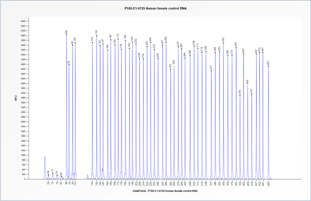
Figure 2. Capillary electrophoresis pattern from a sample of approximately 50 ng human female control DNA analysed with SALSA MLPA Probemix P182 Centromere mix 2 (C1-0725).
