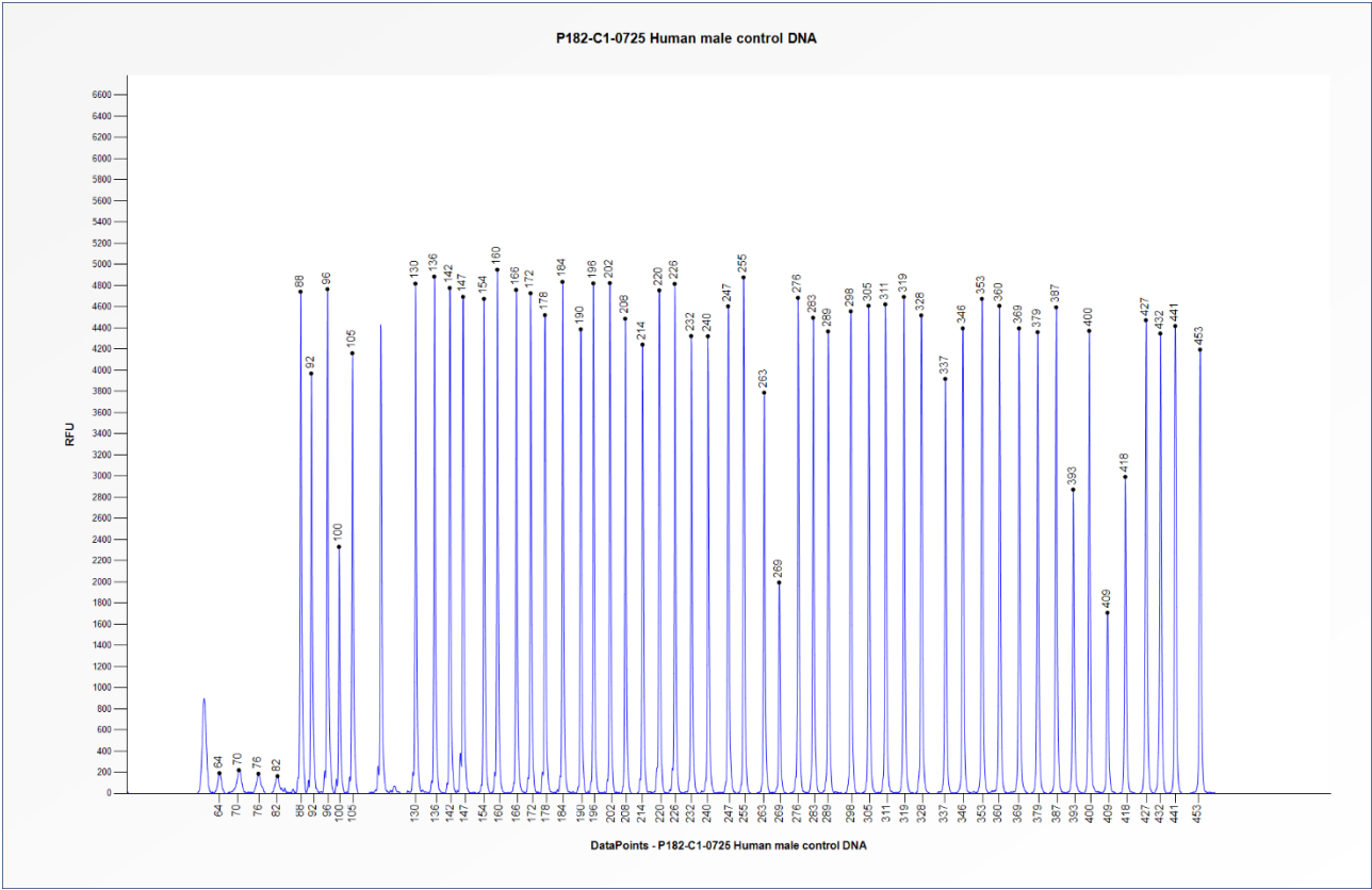
Figure 1. Capillary electrophoresis pattern from a sample of approximately 50 ng human male control DNA analysed with SALSA MLPA Probemix P182 Centromere mix 2 (C1-0725).
