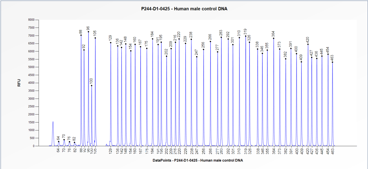
Figure 1. Capillary electrophoresis pattern from a sample of approximately 50 ng human male control DNA analysed with SALSA MLPA Probemix P244 AIP-MEN1-CDKN1B (D1-0425).
