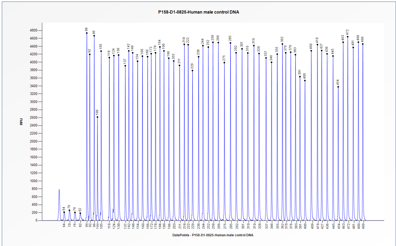
Figure 1. Capillary electrophoresis pattern from a sample of approximately 50 ng human male control DNA analysed with SALSA MLPA Probemix P158 JPS (D1-0825).
