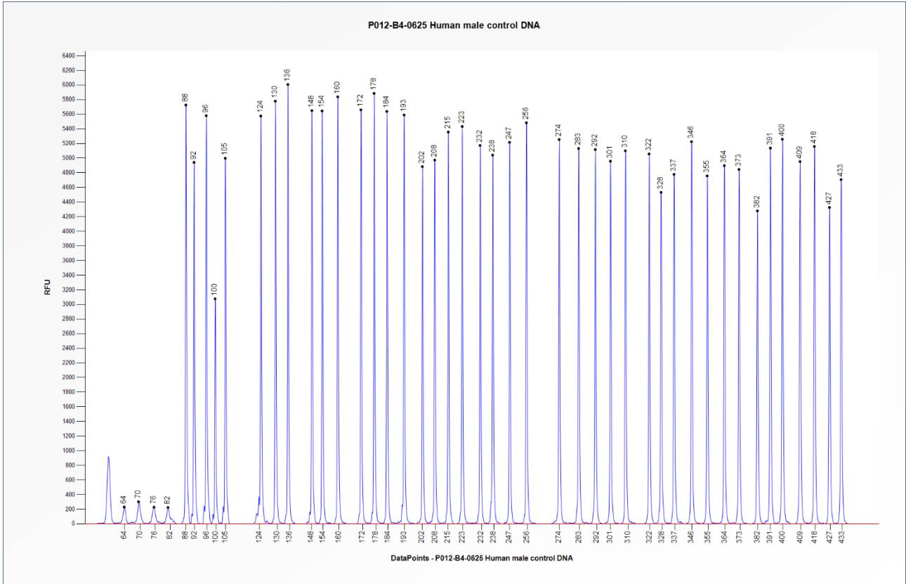
Figure 1. Capillary electrophoresis pattern from a sample of approximately 50 ng human male control DNA analysed with SALSA MLPA Probemix P012 VWF mix 2 (B4-0625).
