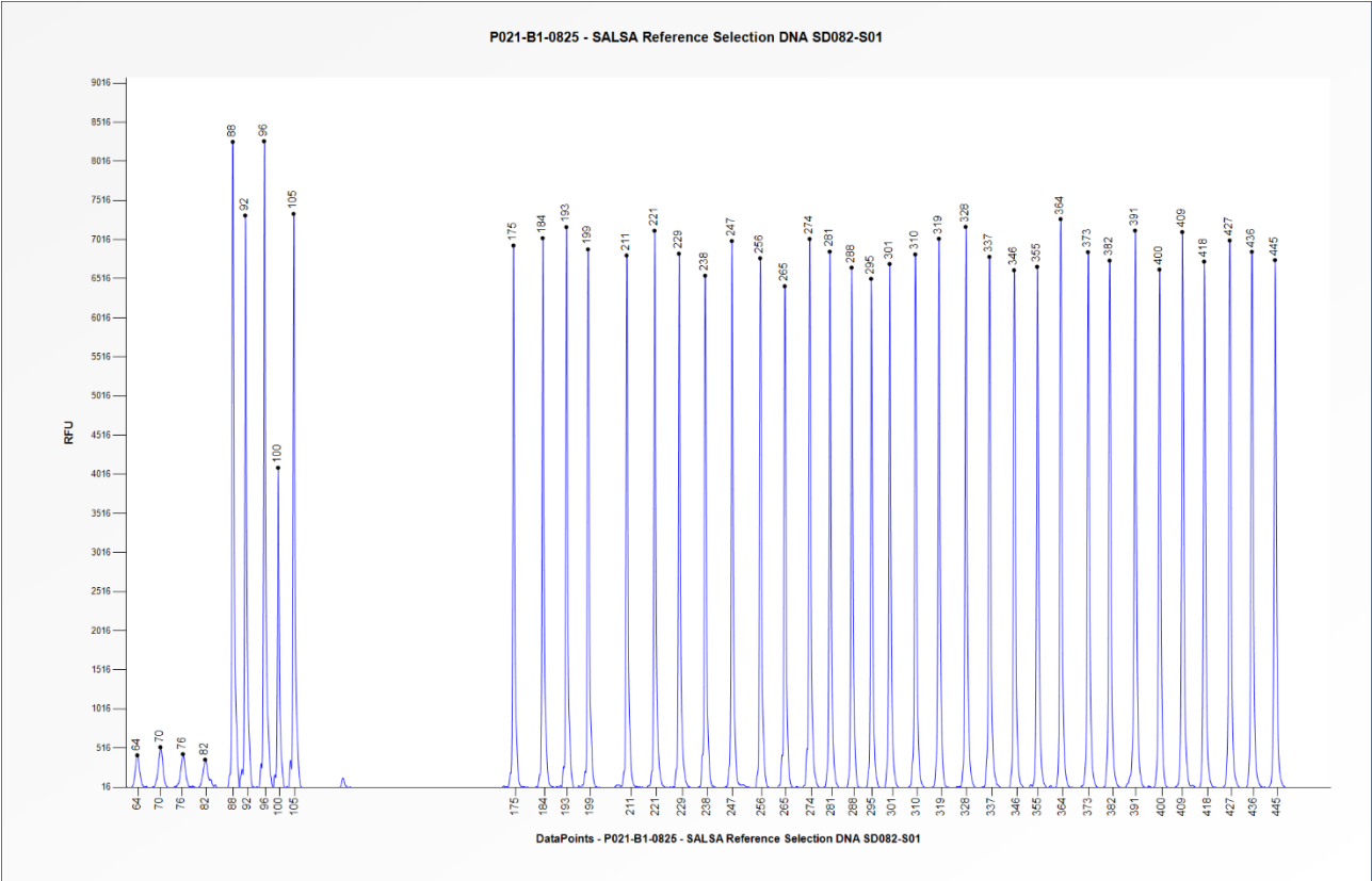
Figure 2. Capillary electrophoresis pattern from SALSA Reference Selection DNA SD082-S01 (approximately 50 ng) analysed with SALSA MLPA Probemix P021 SMA (B1-0825).
