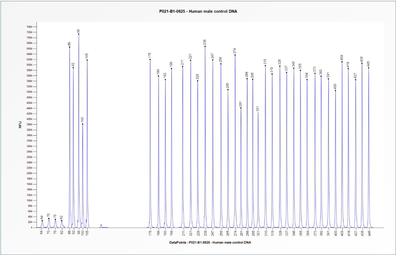
Figure 1. Capillary electrophoresis pattern from a sample of approximately 50 ng human male control DNA analysed with SALSA MLPA Probemix P021 SMA (B1-0825).
