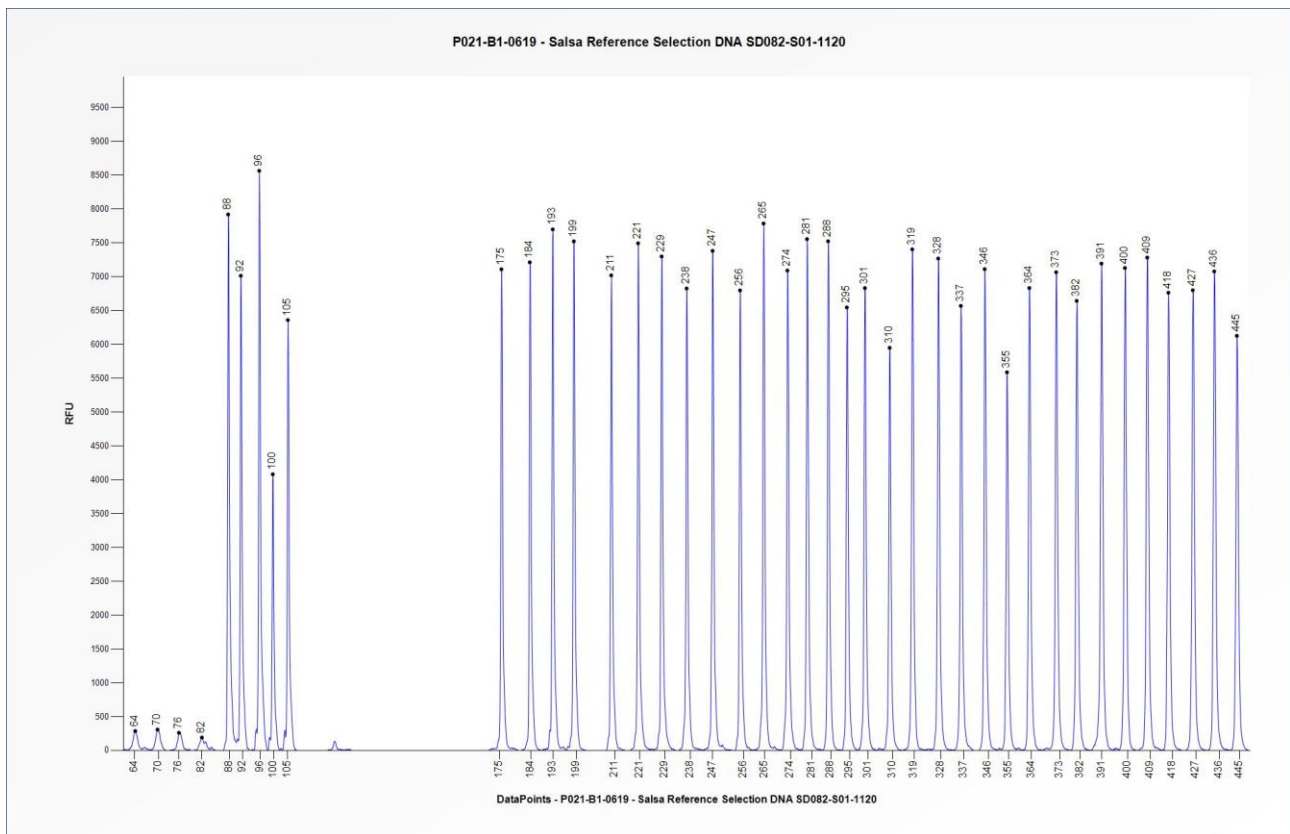
Figure 2. Capillary electrophoresis pattern from SALSA Reference Selection DNA SD082-S01-1120 (approximately 50 ng) analysed with SALSA MLPA Probemix P021 SMA (B1-0619). Probe peak heights may vary between different lots of the P021-B1 probemix.
