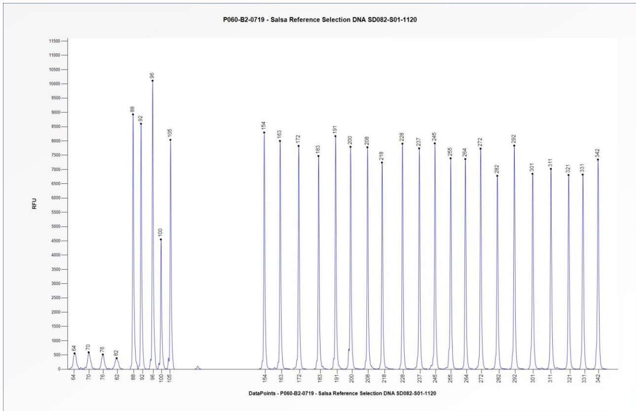
Figure 3. Capillary electrophoresis pattern from SALSA Reference Selection DNA SD082-S01-1120 (approximately 50 ng) analysed with SALSA MLPA Probemix P060 SMA Carrier (B2-0719). Probe peak heights may vary between different lots of the P060-B2 probemix.
