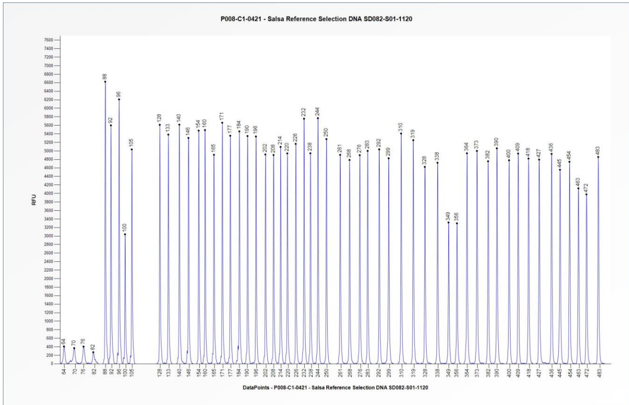
Figure 1. Capillary electrophoresis pattern from SALSA Reference Selection DNA SD082-S01-1120 (approximately 50 ng) analysed with SALSA MLPA Probemix P008 PMS2 (C1-0421). Probe peak heights may vary between different lots of the P008-C1 probemix.
