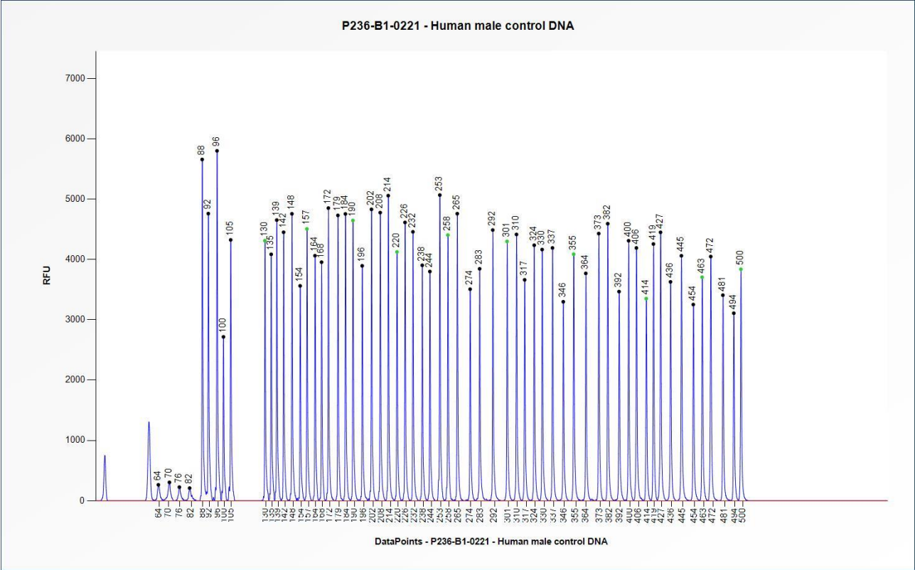
Figure 1. Capillary electrophoresis pattern from a sample of approximately 50 ng human male control DNA analysed with SALSA MLPA Probemix P236 CFH Region (B1-0221).
