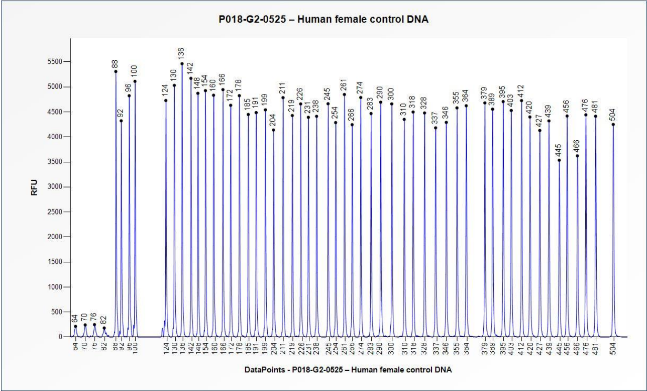
Figure 2. Capillary electrophoresis pattern from a sample of approximately 50 ng human female control DNA analysed with SALSA MLPA Probemix P018 SHOX (G2-0525).
