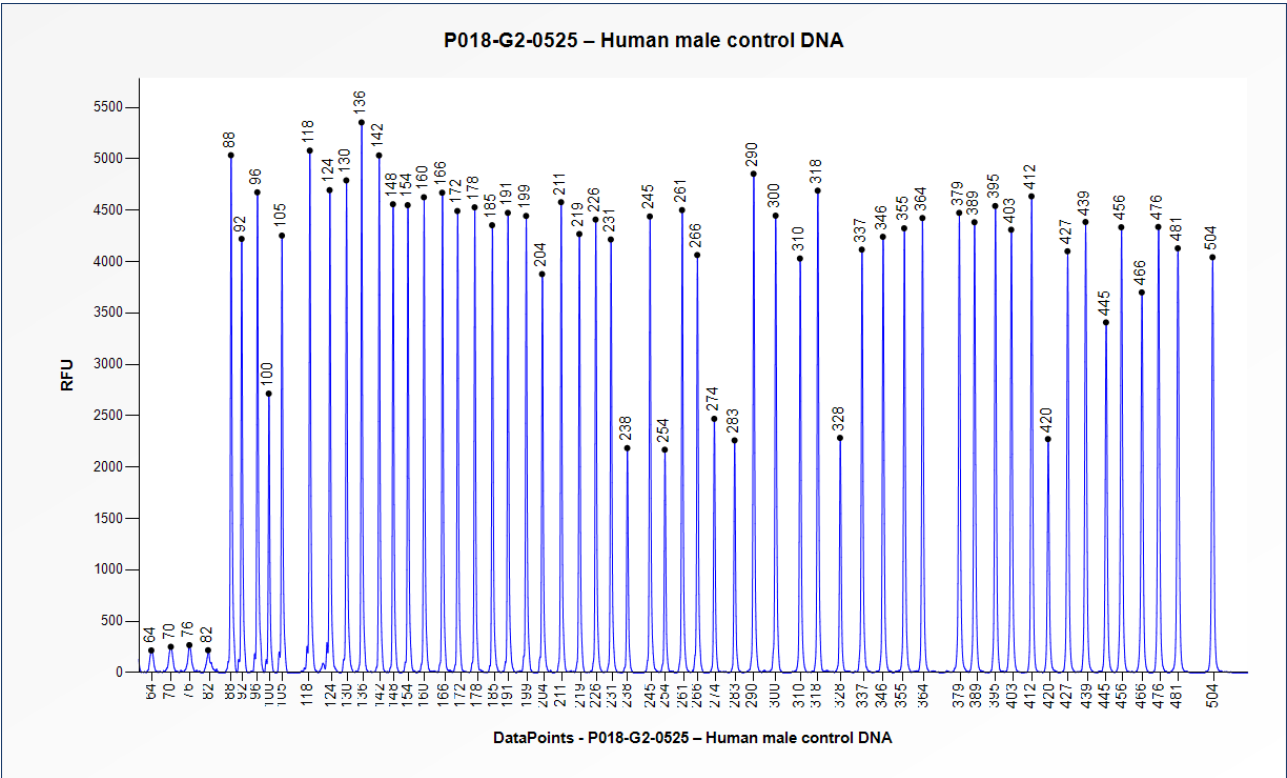
Figure 1. Capillary electrophoresis pattern from a sample of approximately 50 ng human male control DNA analysed with SALSA MLPA Probemix P018 SHOX (G2-0525).
