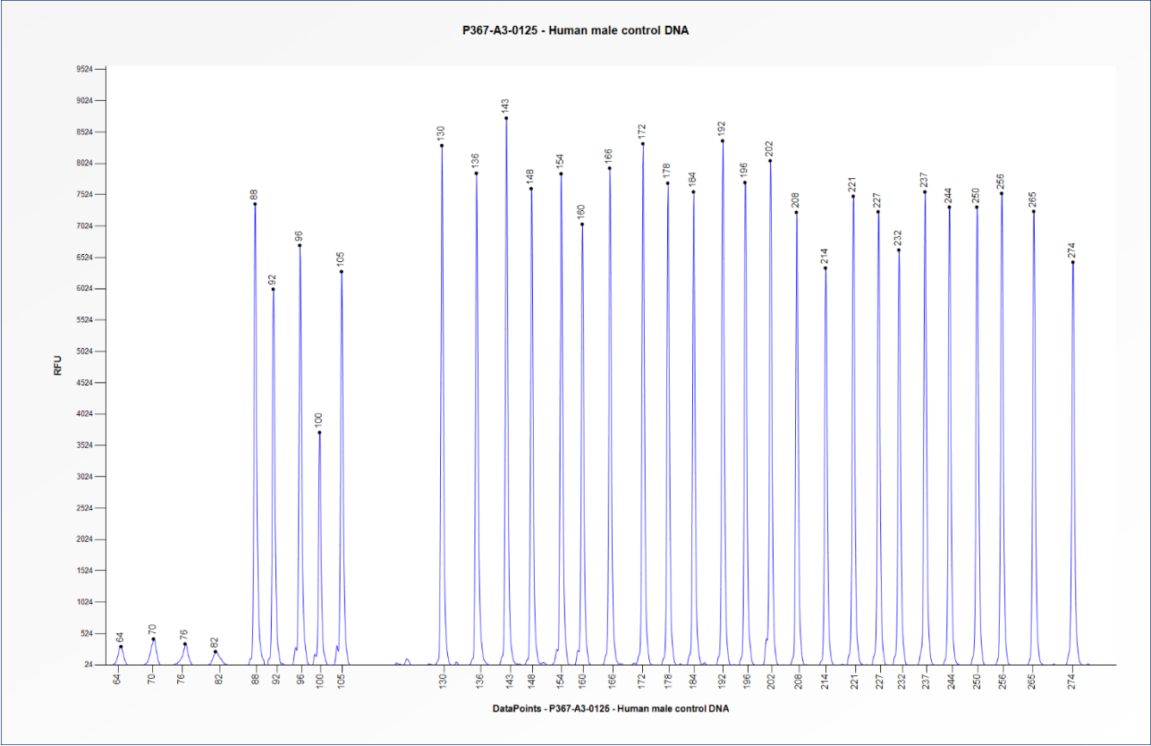
Figure 1. Capillary electrophoresis pattern from a sample of approximately 50 ng human male control DNA analysed with SALSA MLPA Probemix P367 BEST1-PRPH2 (A3-0125).
