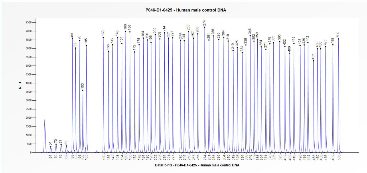
Figure 1. Capillary electrophoresis pattern from a sample of approximately 50 ng human male control DNA analysed with SALSA MLPA Probemix P046 TSC2 (D1-0425).
