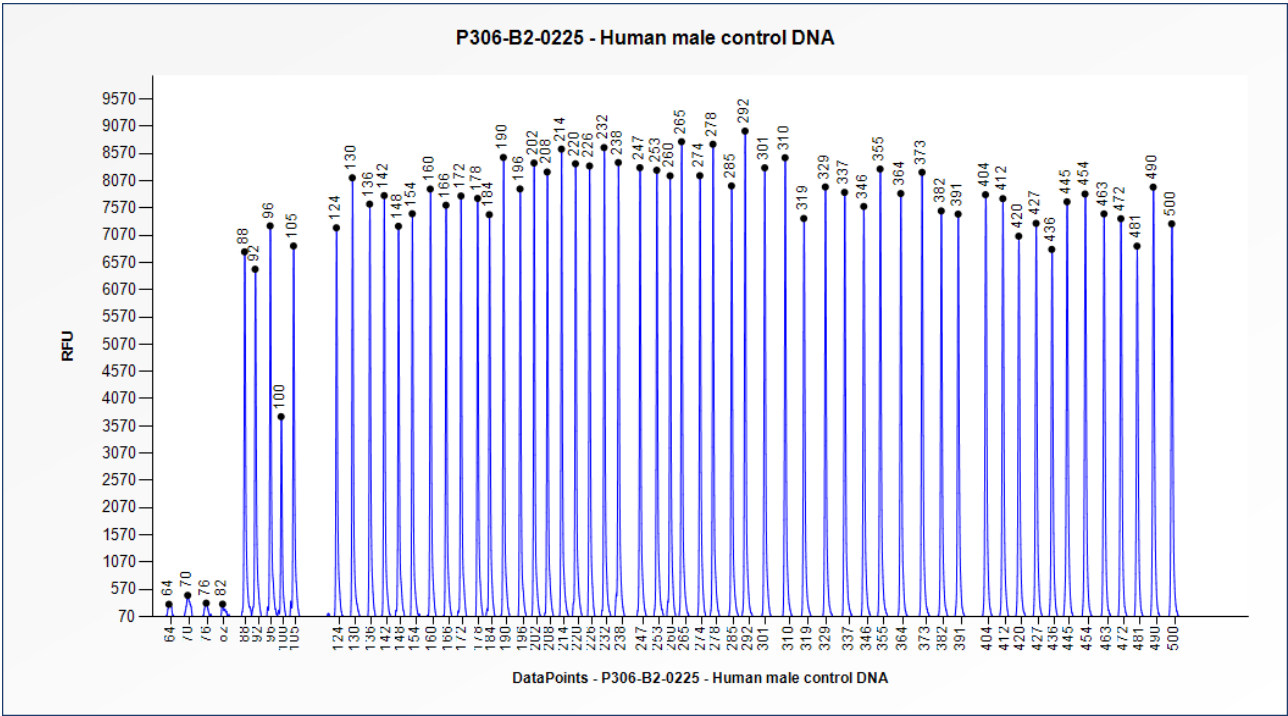
Figure 1. Capillary electrophoresis pattern from a sample of approximately 50 ng human male control DNA analysed with SALSA MLPA Probemix P306 SPG11 (B2-0225).
