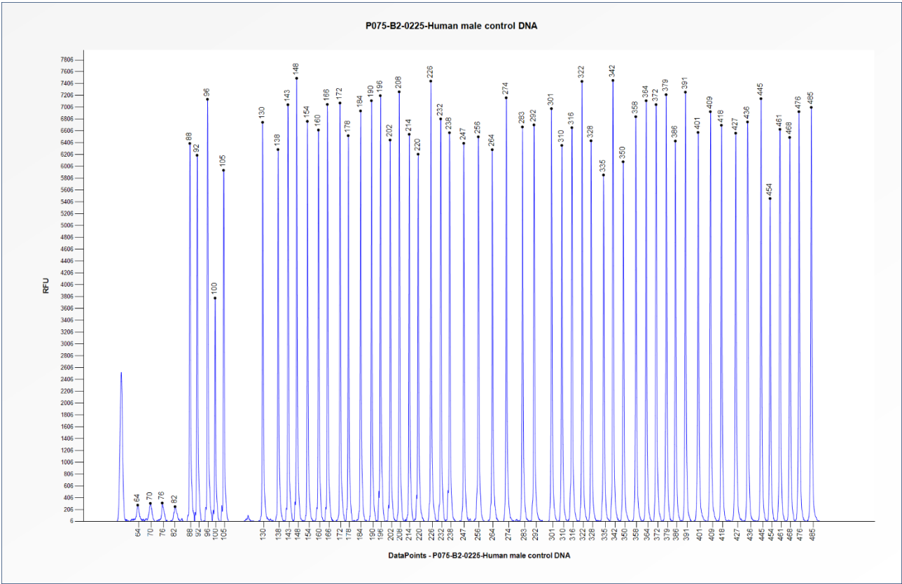
Figure 1. Capillary electrophoresis pattern from a sample of approximately 50 ng human male control DNA analysed with SALSA MLPA Probemix P075 TCF4-FOXG1 (B2-0225).
