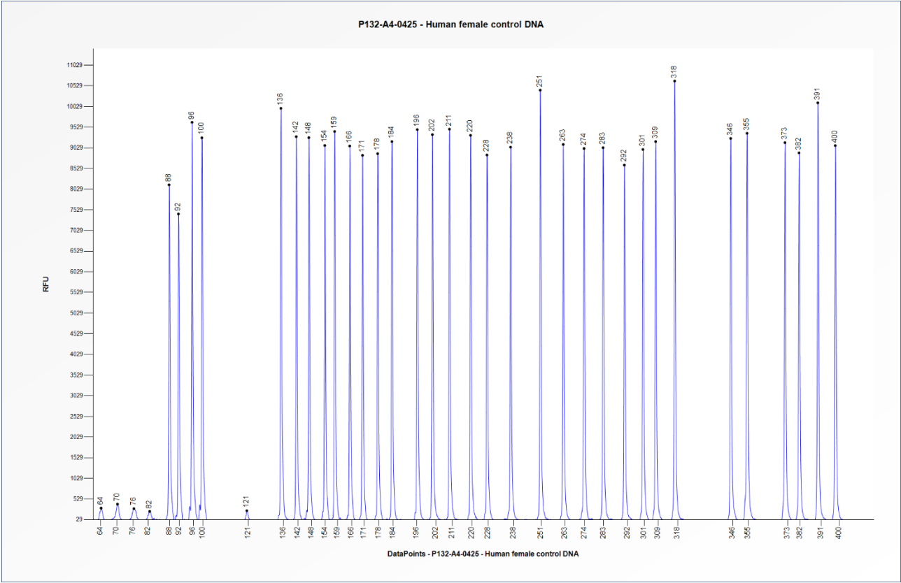
Figure 2. Capillary electrophoresis pattern from a sample of approximately 50 ng human female control DNA analysed with SALSA MLPA Probemix P132 Kallmann-1 (A4-0425).
