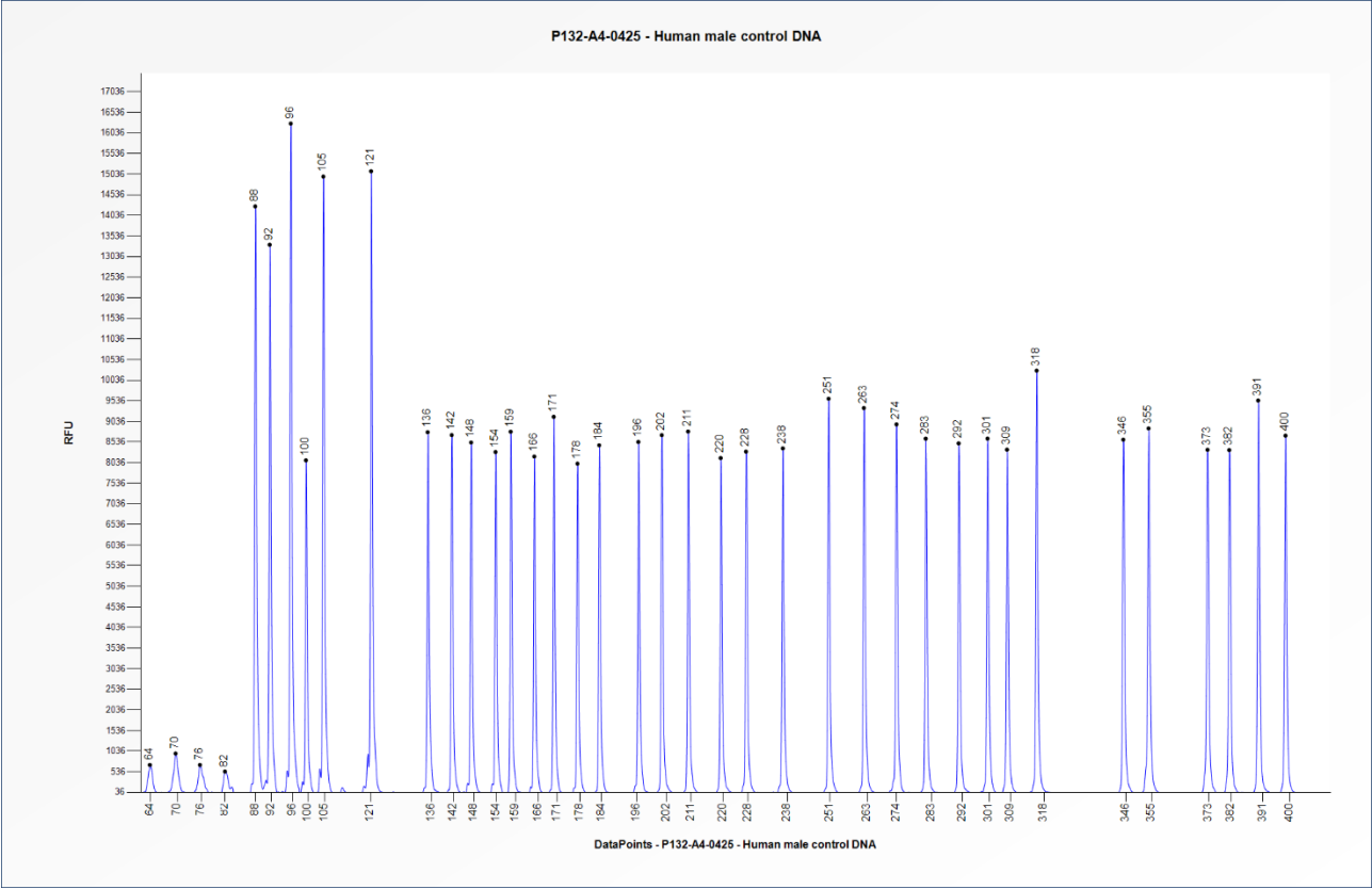
Figure 1. Capillary electrophoresis pattern from a sample of approximately 50 ng human male control DNA analysed with SALSA MLPA Probemix P132 Kallmann-1 (A4-0425).
