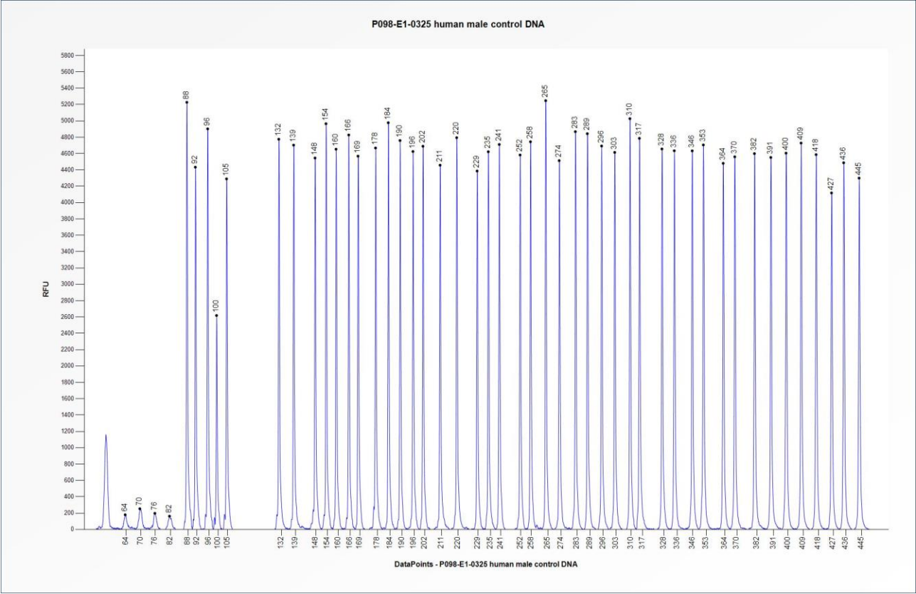
Figure 1. Capillary electrophoresis pattern from a sample of approximately 50 ng human male control DNA analysed with SALSA MLPA Probemix P098 Wilson disease (E1-0325).
