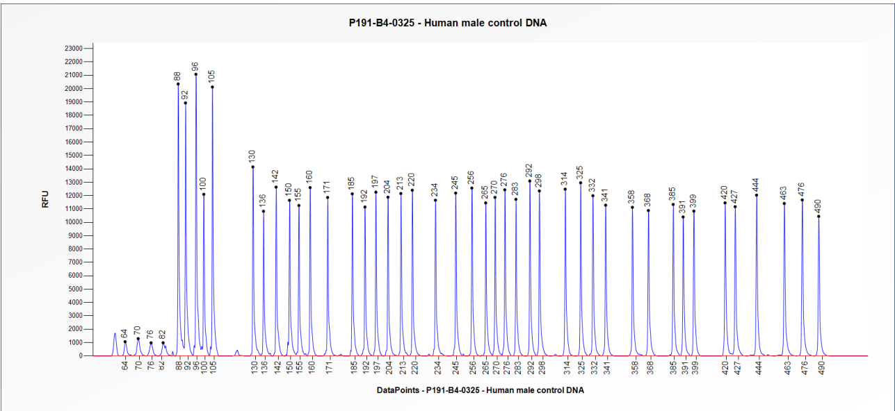
Figure 1. Capillary electrophoresis pattern from a sample of approximately 50 ng human male control DNA analysed with SALSA MLPA Probemix P191 X-linked Alport syndrome mix 1 (B4-0325).
