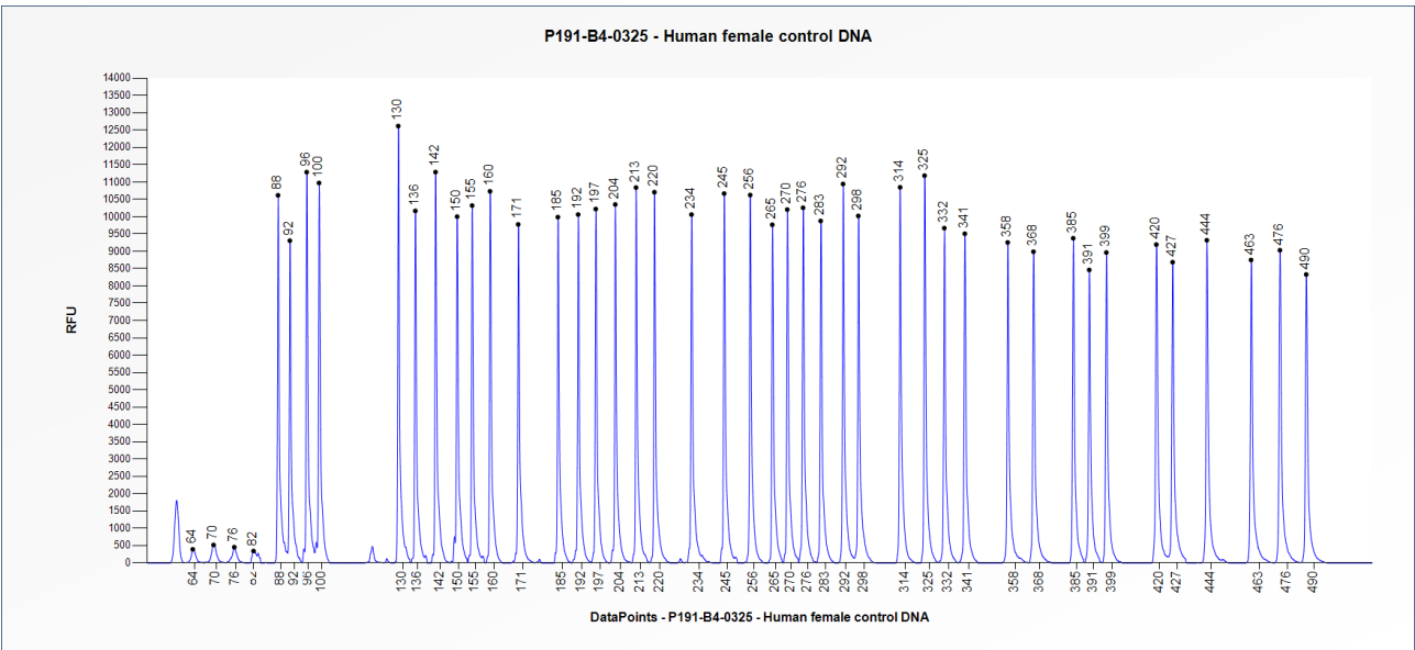
Figure 2. Capillary electrophoresis pattern from a sample of approximately 50 ng human female control DNA analysed with SALSA MLPA Probemix P191 X-linked Alport syndrome mix 1 (B4-0325).
