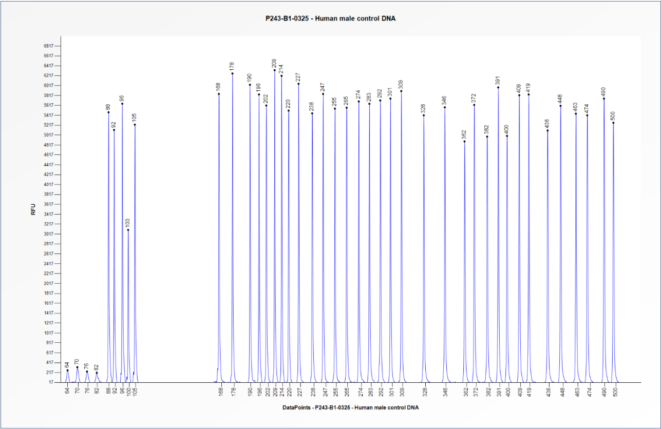
Figure 1. Capillary electrophoresis pattern from a sample of approximately 50 ng human male control DNA analysed with SALSA MLPA Probemix P243 SERPING1 - F12 (B1-0325).
