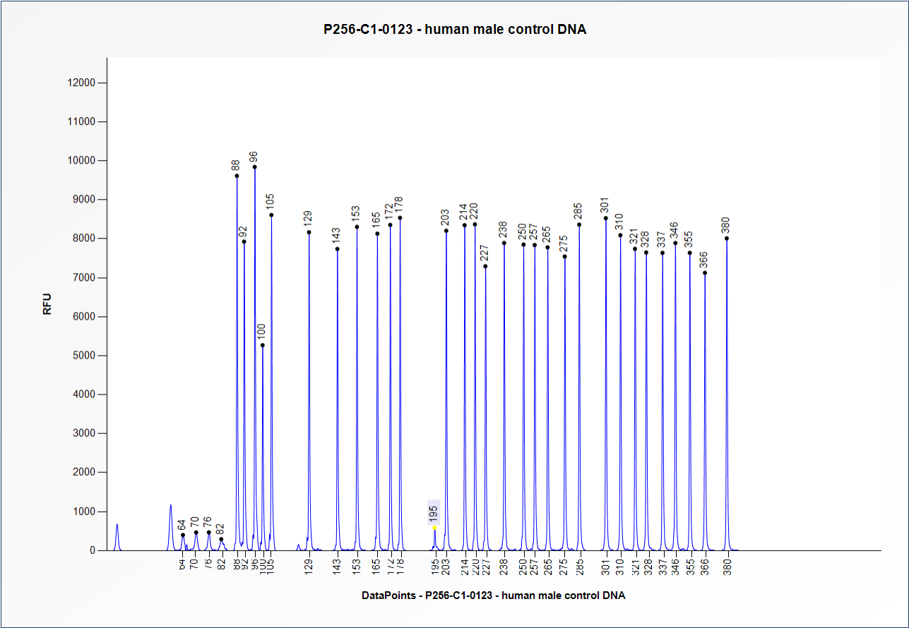
Figure 1. Capillary electrophoresis pattern from a sample of approximately 50 ng human male control DNA analysed with SALSA MLPA Probemix P256 FLCN (C1-0123). Please note that in healthy samples without the c.1285dupC mutation, the FLCN 195 nt probe will generate a background signal of 5-10% of the median peak height of all reference probes, which indicates absence of the mutation.
