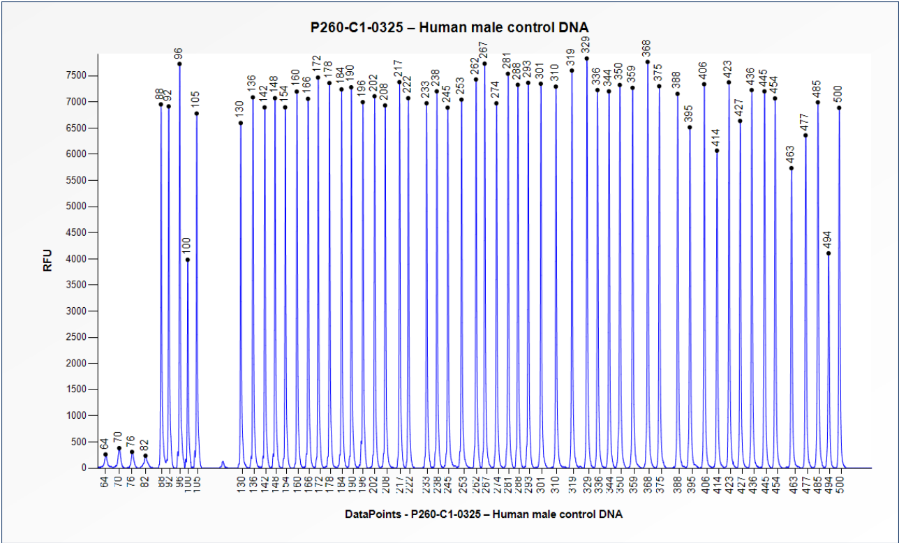
Figure 1. Capillary electrophoresis pattern from a sample of approximately 50 ng human male control DNA analysed with SALSA MLPA Probemix P260 PALB2-RAD50-RAD51C-RAD51D (C1-0325).
