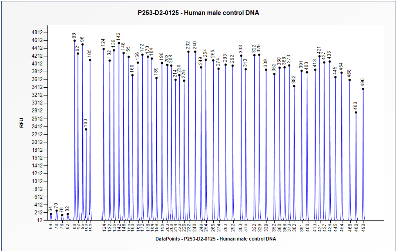
Figure 1. Capillary electrophoresis pattern from a sample of approximately 50 ng human male control DNA analysed with SALSA MLPA Probemix P253 NB mix 3 (D2-0125).
