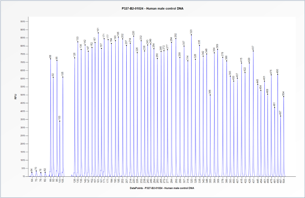
Figure 1. Capillary electrophoresis pattern from a sample of approximately 50 ng human male control DNA analysed with SALSA MLPA Probemix P327 iAMP21-ERG (B2-1024).
