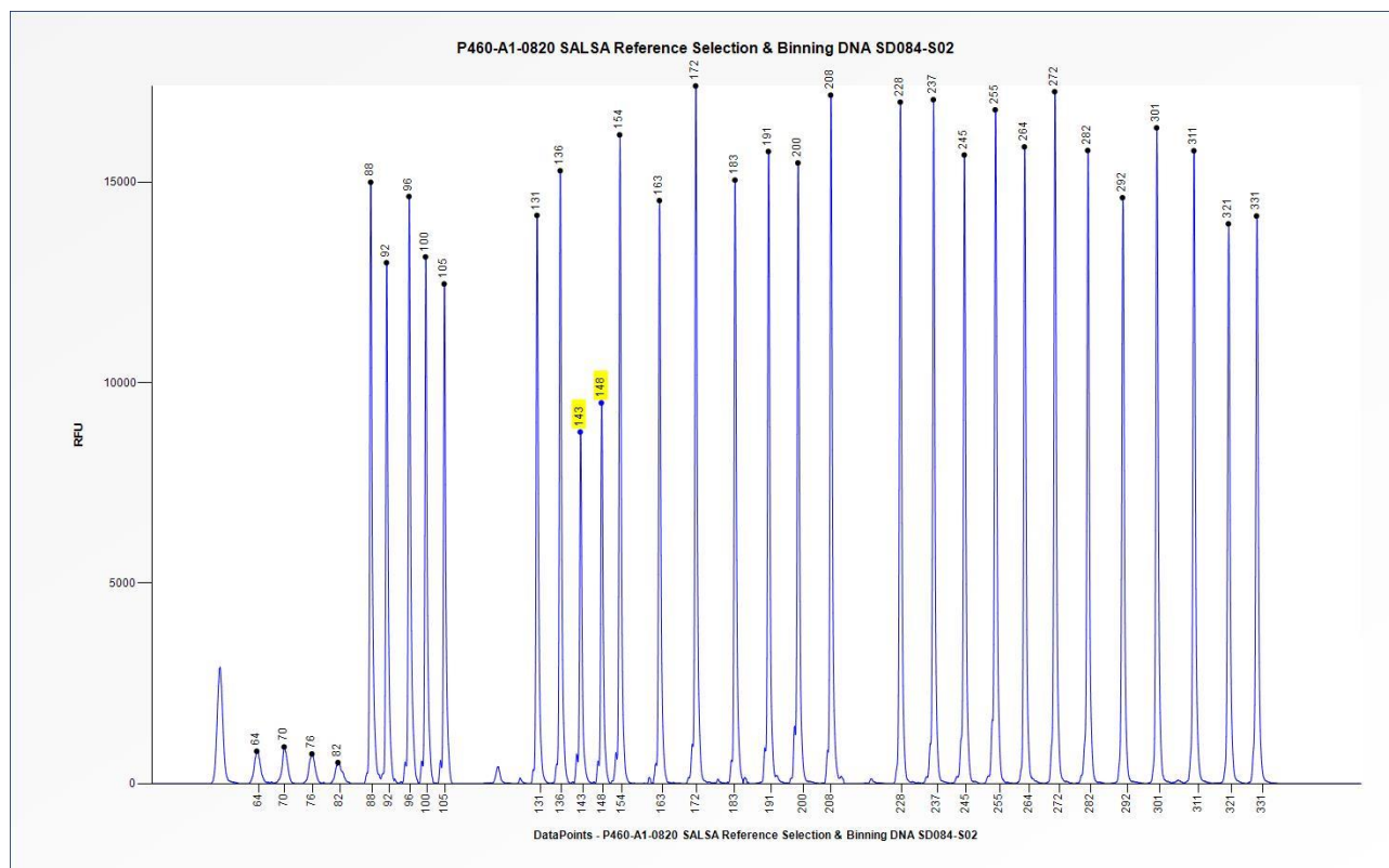
Figure 2. Capillary electrophoresis pattern from SALSA Reference Selection & Binning DNA SD084-S02 (approximately 50 ng) analysed with SALSA MLPA Probemix P460 SMA (Silent) Carrier (A1-0820). The locations of the g.27134T>G and g.27706-27707delAT specific probes, at 143 nt and 148 nt respectively, are indicated.
