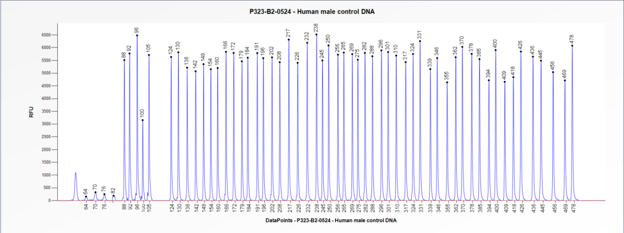
Figure 1. Capillary electrophoresis pattern from a sample of approximately 50 ng human male control DNA analysed with SALSA MLPA Probemix P323-B2 CDK4-HMGA2-MDM2 (B2-0524).
