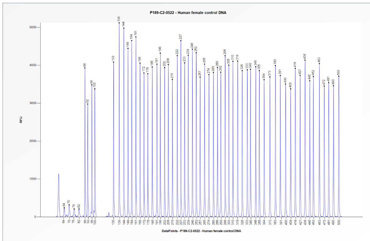
Figure 2. Capillary electrophoresis pattern from a sample of approximately 50 ng human female control DNA analysed with SALSA MLPA Probemix P189 CDKL5/ARX/FOXG1 (C2-0522).
