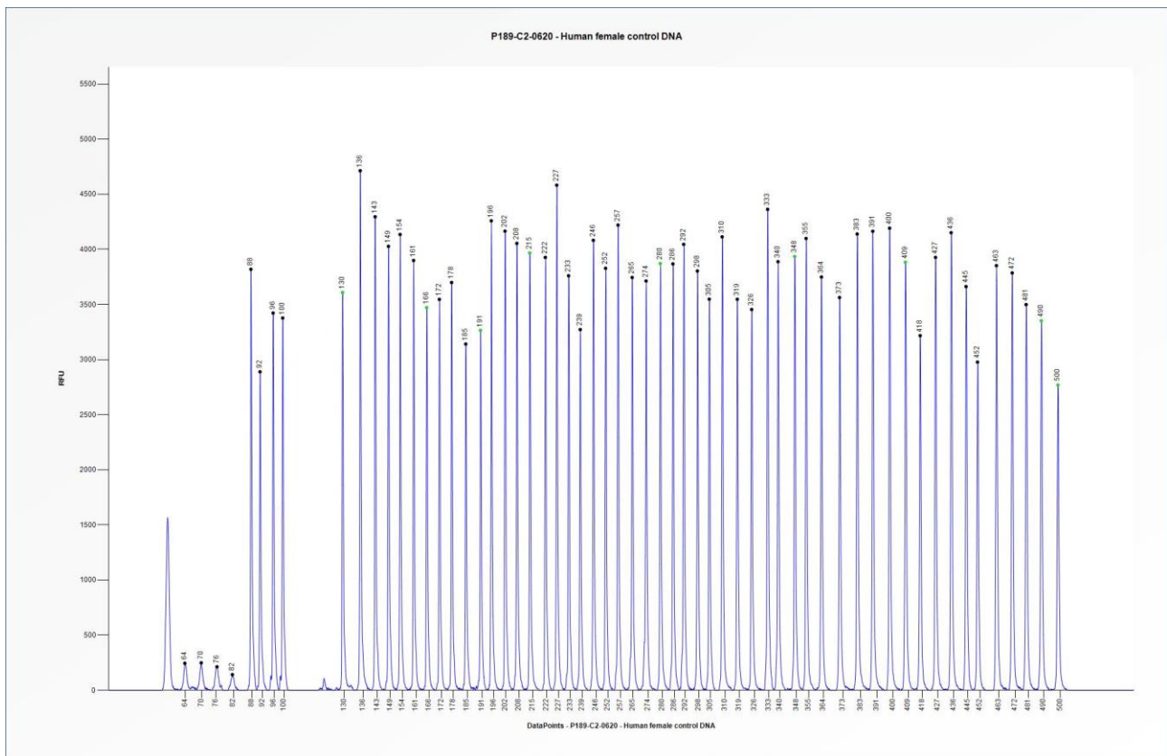
Figure 2. Capillary electrophoresis pattern from a sample of approximately 50 ng human female control DNA analysed with SALSA MLPA Probemix P189 CDKL5/ARX/FOXG1 (C2-0620).
