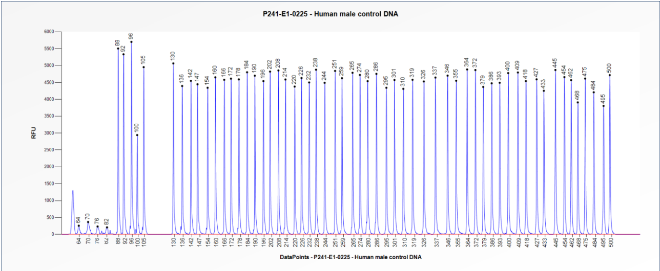
Figure 1. Capillary electrophoresis pattern from a sample of approximately 50 ng human male control DNA analysed with SALSA MLPA Probemix P241 MODY Mix 1 (E1-0225).
