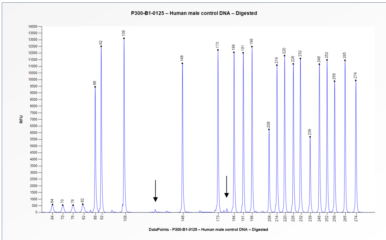
Figure 2. Capillary electrophoresis pattern from a sample of approximately 50 ng digested human male control DNA analysed with SALSA MLPA Probemix P300 Reference-2 (B1-0125) to determine the methylation status. Digestion control probes are indicated with arrows.
