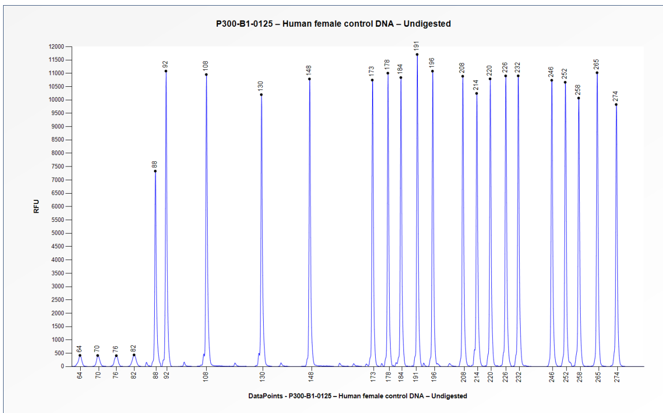
Figure 3. Capillary electrophoresis pattern from a sample of approximately 50 ng undigested human female control DNA analysed with SALSA MLPA Probemix P300 Reference-2 (B1-0125) for the quantification of copy numbers.
