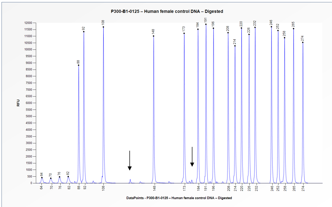
Figure 4. Capillary electrophoresis pattern from a sample of approximately 50 ng digested human female control DNA analysed with SALSA MLPA Probemix P300 Reference-2 (B1-0125) to determine the methylation status. Digestion control probes are indicated with arrows.
