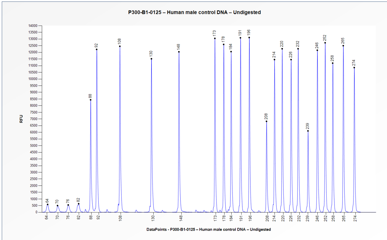
Figure 1. Capillary electrophoresis pattern from a sample of approximately 50 ng undigested human male control DNA analysed SALSA MLPA Probemix P300 Reference-2 (B1-0125) for the quantification of copy numbers.
