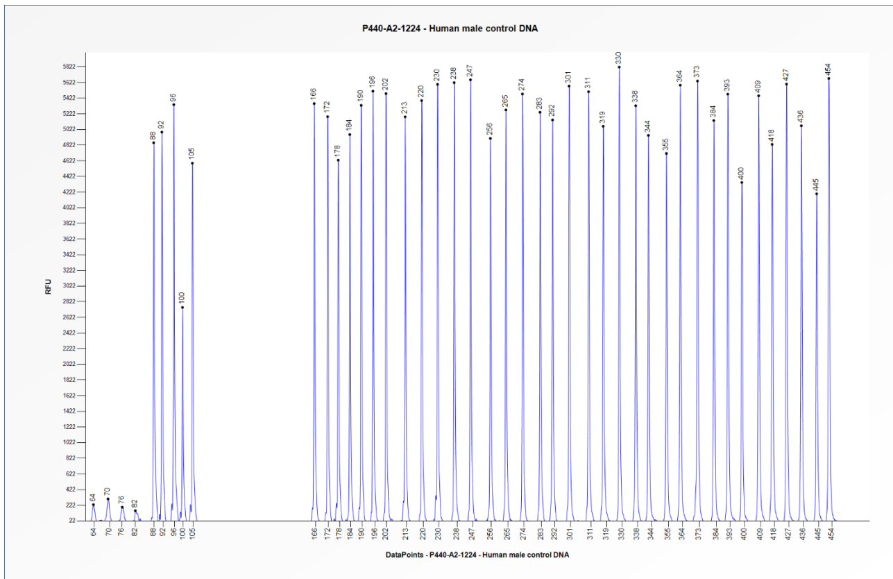
Figure 1. Capillary electrophoresis pattern from a sample of approximately 50 ng human male control DNA analysed with SALSA MLPA Probemix P440 F10 + F11 (A2-1224).
