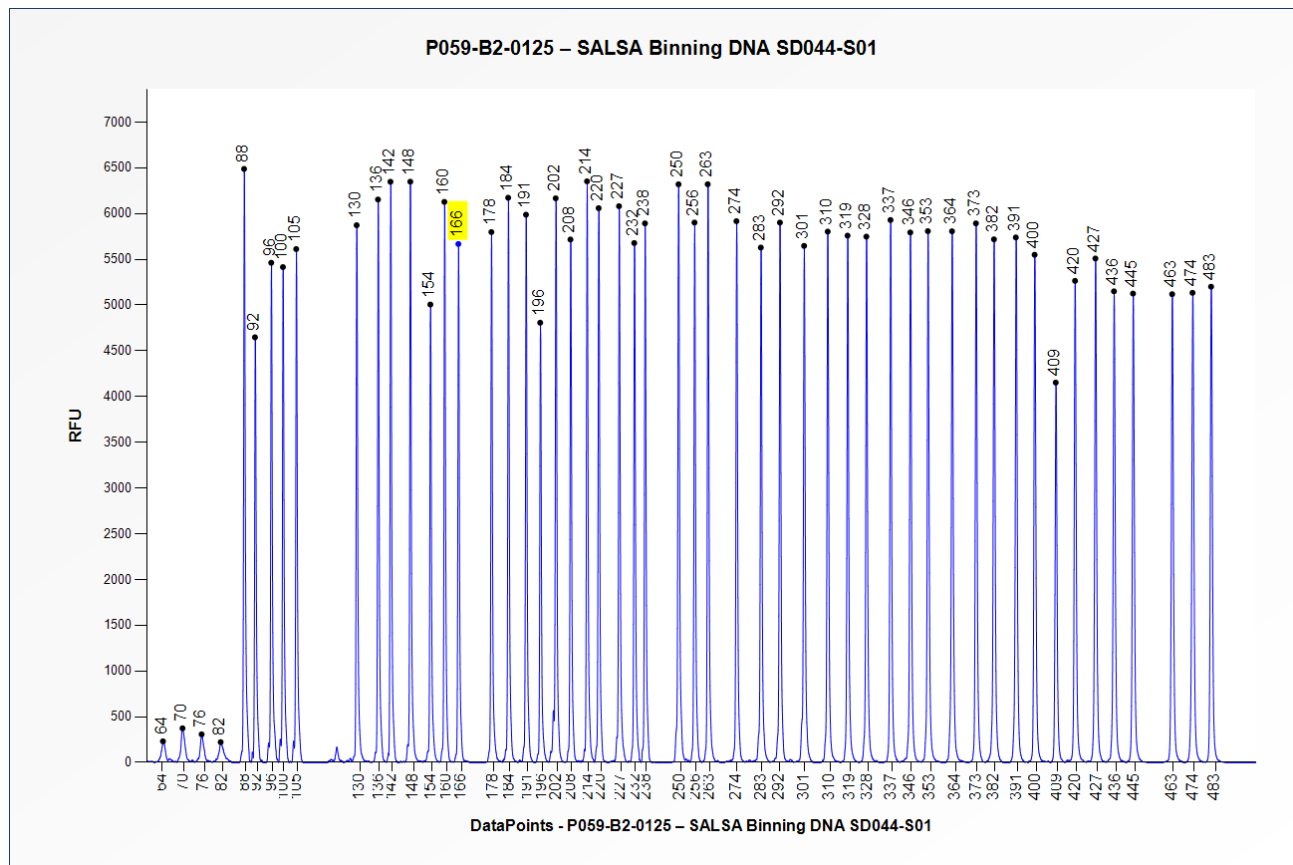
Figure 2. Capillary electrophoresis pattern from SALSA Binning DNA SD044-S01 (approximately 50 ng) analysed with SALSA MLPA Probemix P059 Dystonia (B2-0125). The location of the c.907_909delGAG mutation specific probe at 166 nt is indicated.
