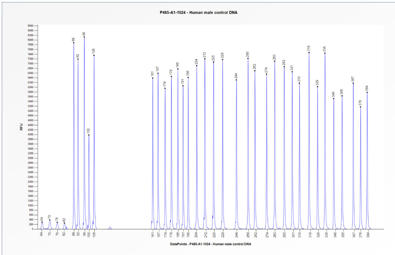
Figure 1. Capillary electrophoresis pattern from a sample of approximately 50 ng human male control DNA analysed with SALSA MLPA Probemix P465 ACADM (A1-1024).
