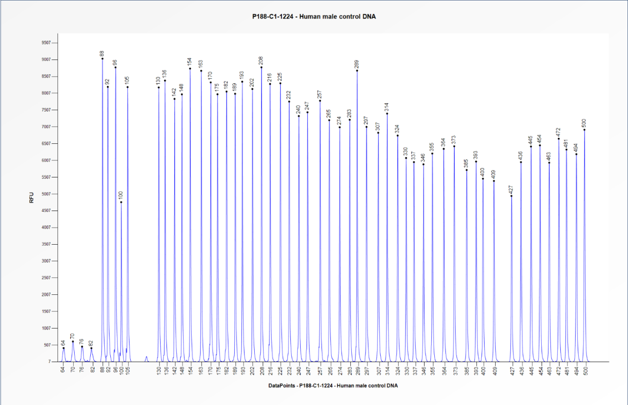
Figure 1. Capillary electrophoresis pattern from a sample of approximately 50 ng human male control DNA analysed with SALSA MLPA Probemix P188 22q13 (C1-1224).
