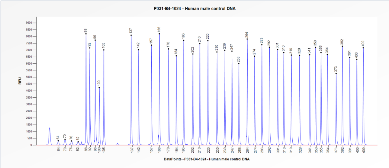
Figure 1. Capillary electrophoresis pattern from a sample of approximately 50 ng human male control DNA analysed with SALSA MLPA Probemix P031 FANCA mix 1 (B4-1024).
