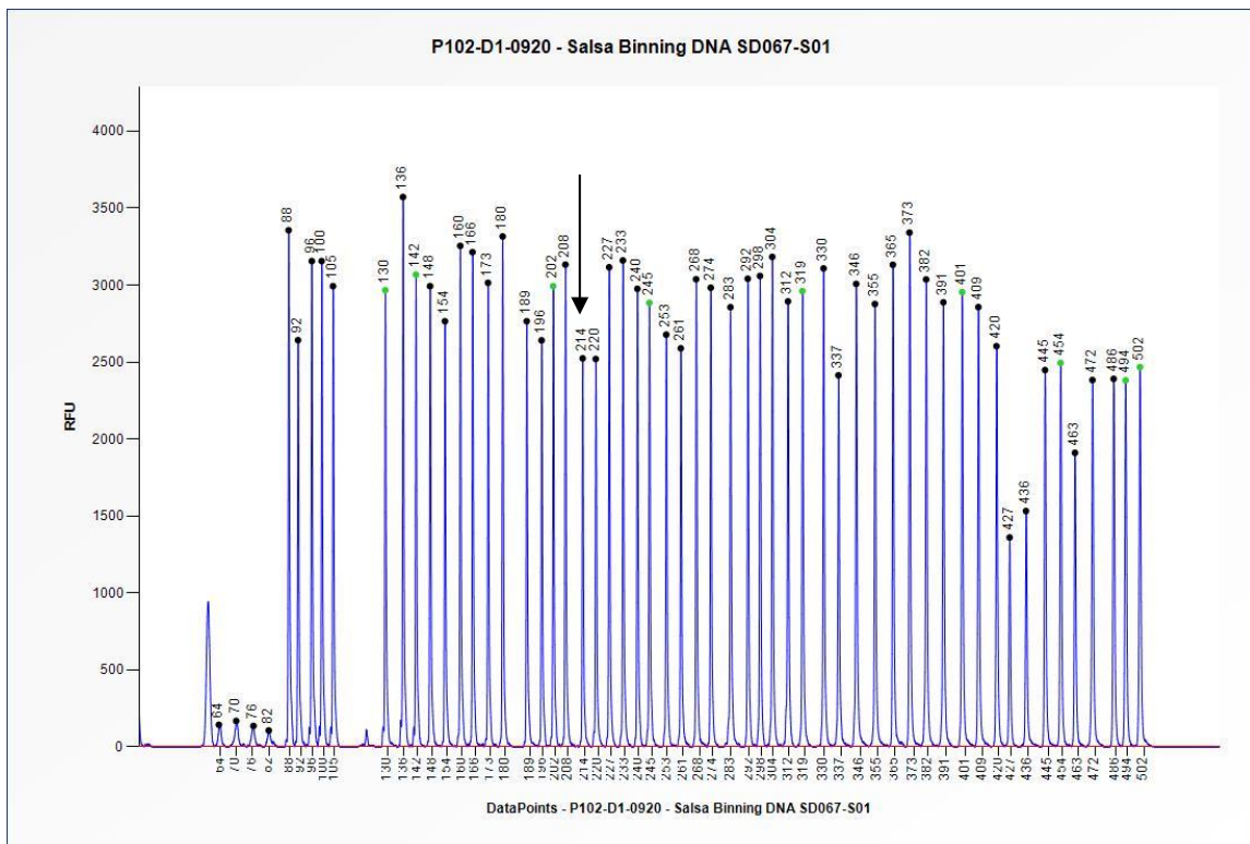
Figure 2. Capillary electrophoresis pattern from SALSA Binning DNA SD067-S01 (approximately 50 ng) analysed with SALSA MLPA probemix P102 HBB (D1-0920). The location of the haemoglobin S mutation-specific probe at 214 nt is indicated.
