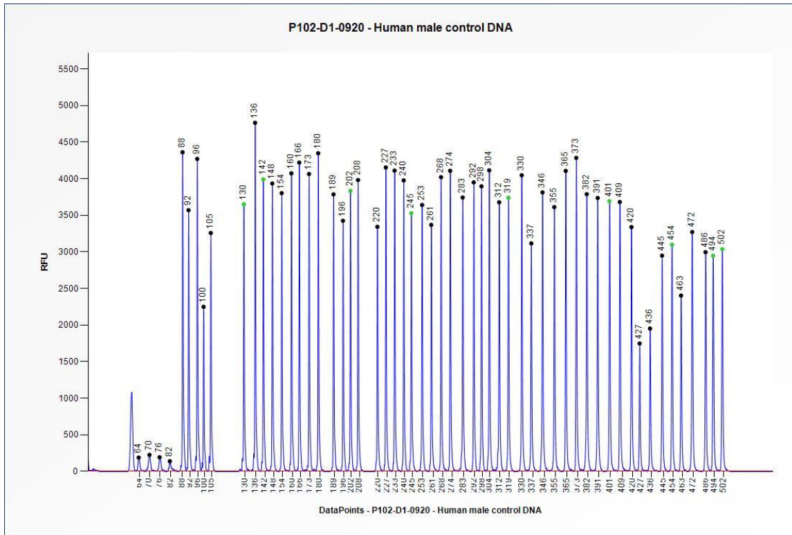
Figure 1. Capillary electrophoresis pattern from a sample of approximately 50 ng human male control DNA analysed with SALSA MLPA Probemix P102 HBB (D1-0920).
